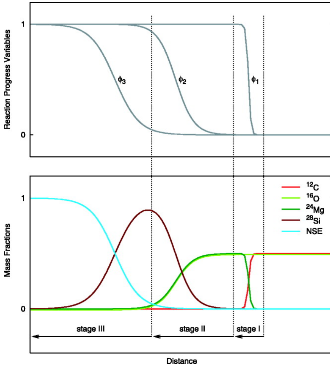
Fig. 6. from Capturing the Fire: Flame Energetics and Neutronization for Type Ia Supernova Simulations Calder et al. 2007 ApJ 656 313 doi:10.1086/510709 https://dx.doi.org/10.1086/510709
