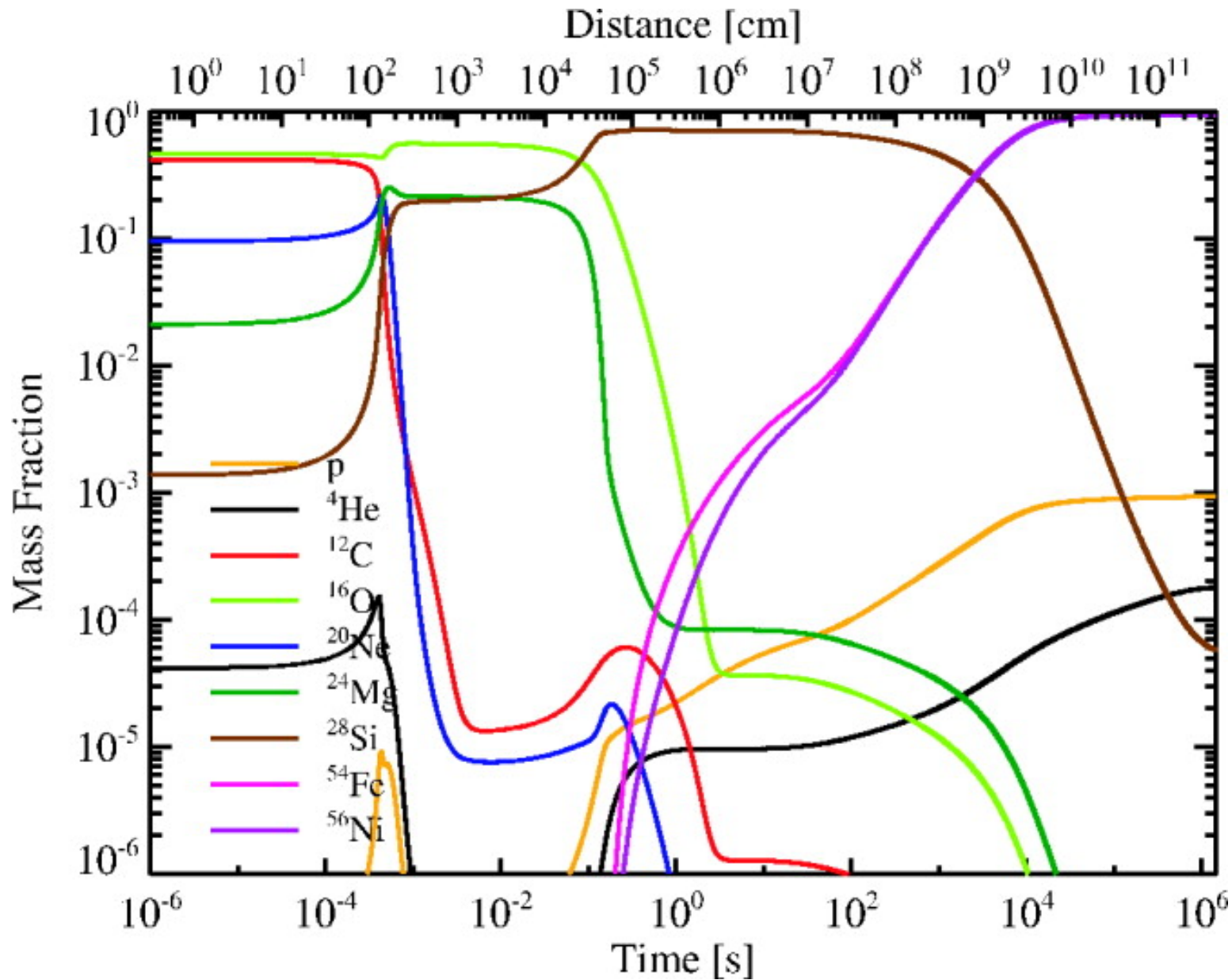
Fig. 4. from Capturing the Fire: Flame Energetics and Neutronization for Type Ia Supernova Simulations Calder et al. 2007 ApJ 656 313 doi:10.1086/510709 https://dx.doi.org/10.1086/510709 © 2007. The American Astronomical Society. All rights reserved. Printed in U.S.A.
