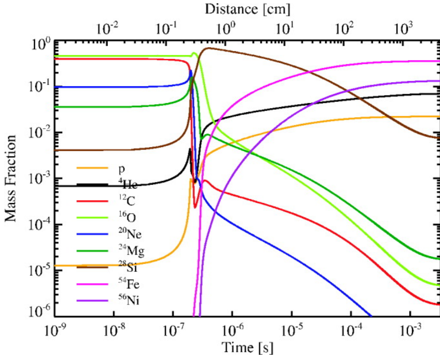
Fig. 3. from Capturing the Fire: Flame Energetics and Neutronization for Type Ia Supernova Simulations Calder et al. 2007 ApJ 656 313 doi:10.1086/510709 https://dx.doi.org/10.1086/510709 © 2007. The American Astronomical Society. All rights reserved. Printed in U.S.A.
