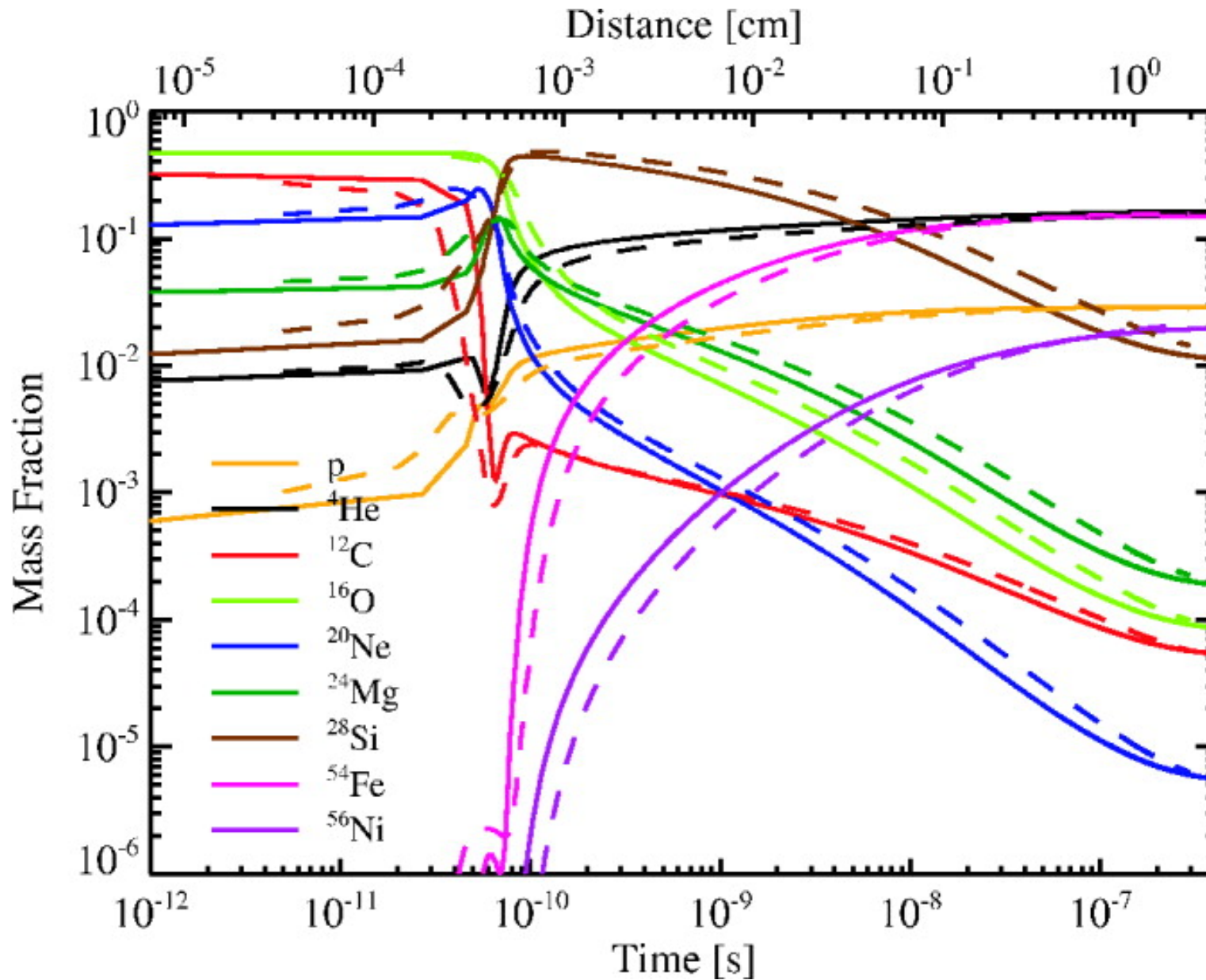
Fig. 2. from Capturing the Fire: Flame Energetics and Neutronization for Type Ia Supernova Simulations Calder et al. 2007 ApJ 656 313 doi:10.1086/510709 https://dx.doi.org/10.1086/510709 © 2007. The American Astronomical Society. All rights reserved. Printed in U.S.A.
