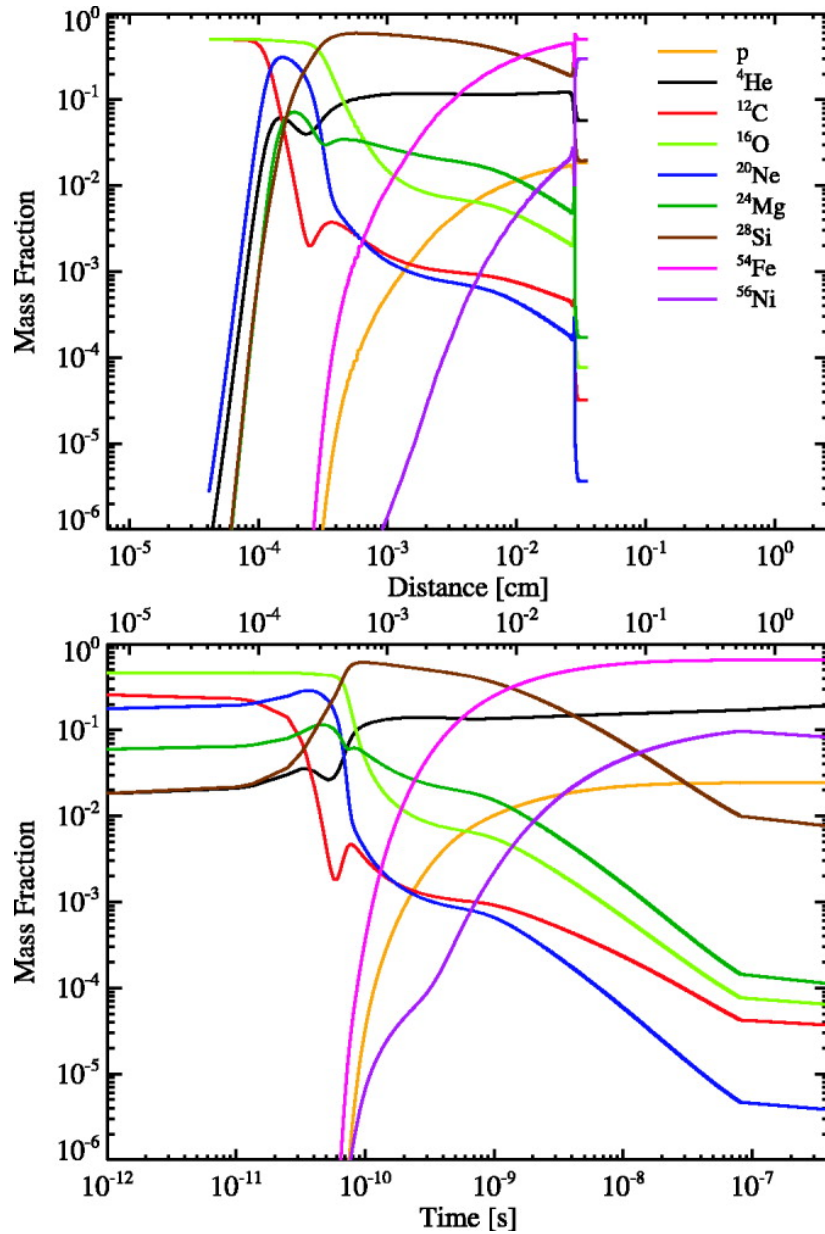
Fig. 1. from Capturing the Fire: Flame Energetics and Neutronization for Type Ia Supernova Simulations Calder et al. 2007 ApJ 656 313 doi:10.1086/510709 https://dx.doi.org/10.1086/510709
