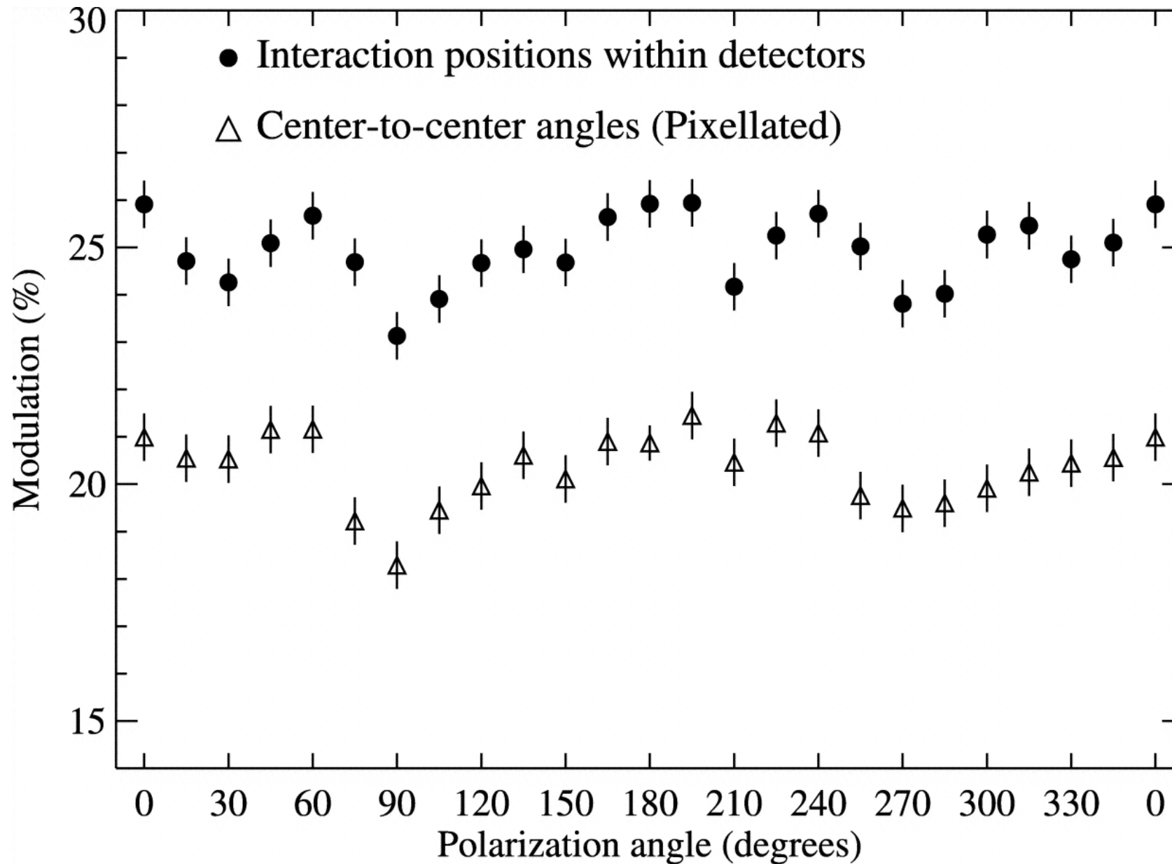
Fig. 8. from Search for Polarization from the Prompt GammaRay Emission of GRB 041219a with SPI on INTEGRAL Kalemci et al. 2007 ApJS 169 75 doi:10.1086/510676 https://dx.doi.org/10.1086/510676
