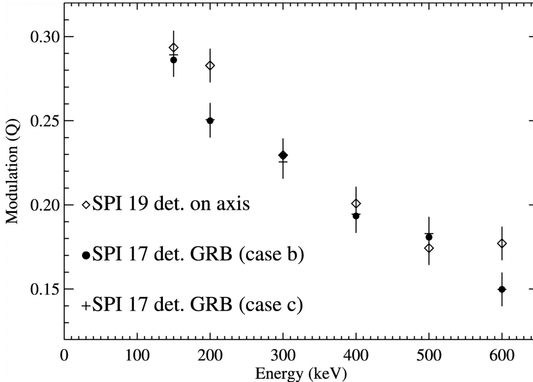
Fig. 7. from Search for Polarization from the Prompt GammaRay Emission of GRB 041219a with SPI on INTEGRAL Kalemci et al. 2007 ApJS 169 75 doi:10.1086/510676 https://dx.doi.org/10.1086/510676 © 2007. The American Astronomical Society. All rights reserved. Printed in U.S.A.
