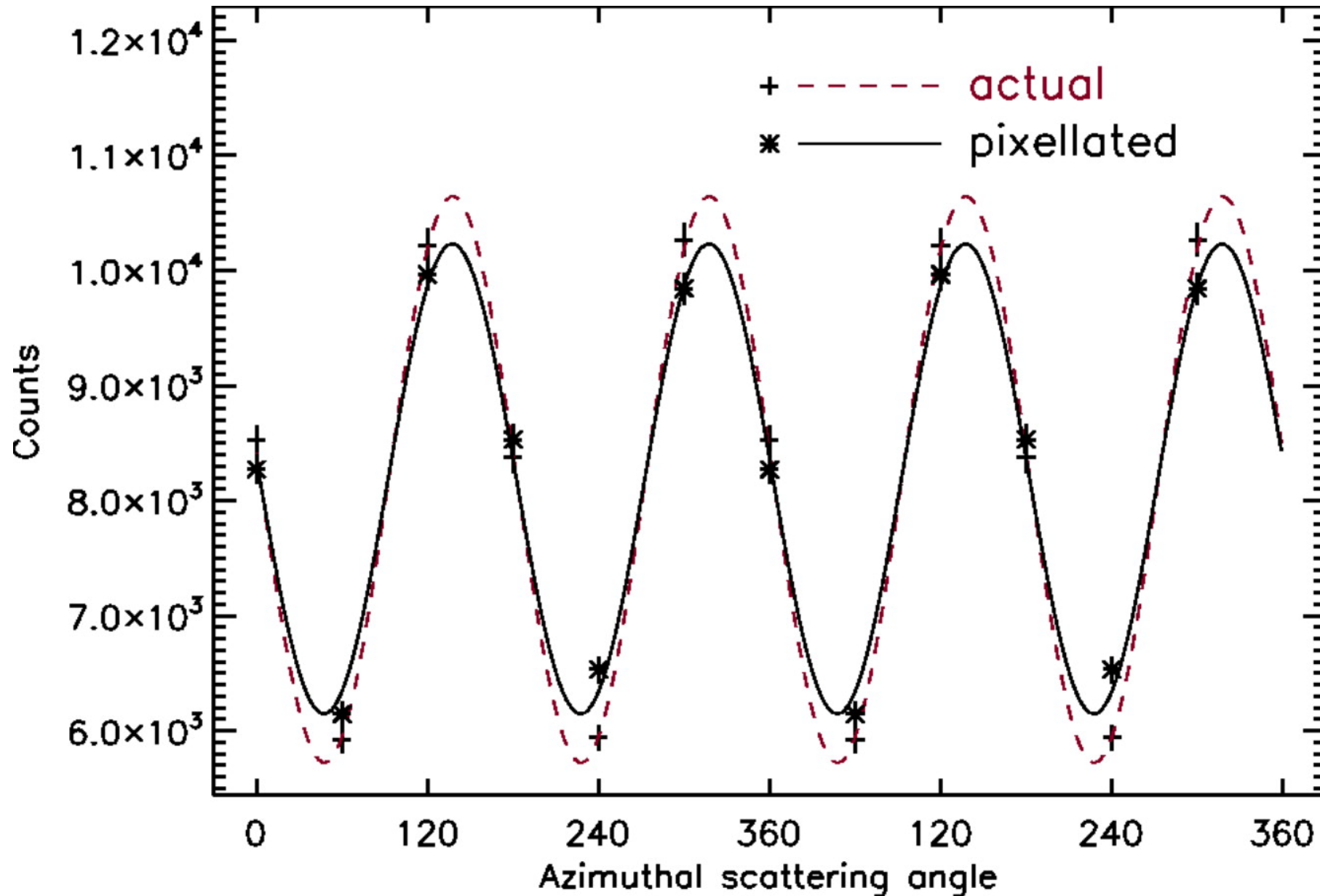
Fig. 6. from Search for Polarization from the Prompt GammaRay Emission of GRB 041219a with SPI on INTEGRAL Kalemci et al. 2007 ApJS 169 75 doi:10.1086/510676 https://dx.doi.org/10.1086/510676 © 2007. The American Astronomical Society. All rights reserved. Printed in U.S.A.
