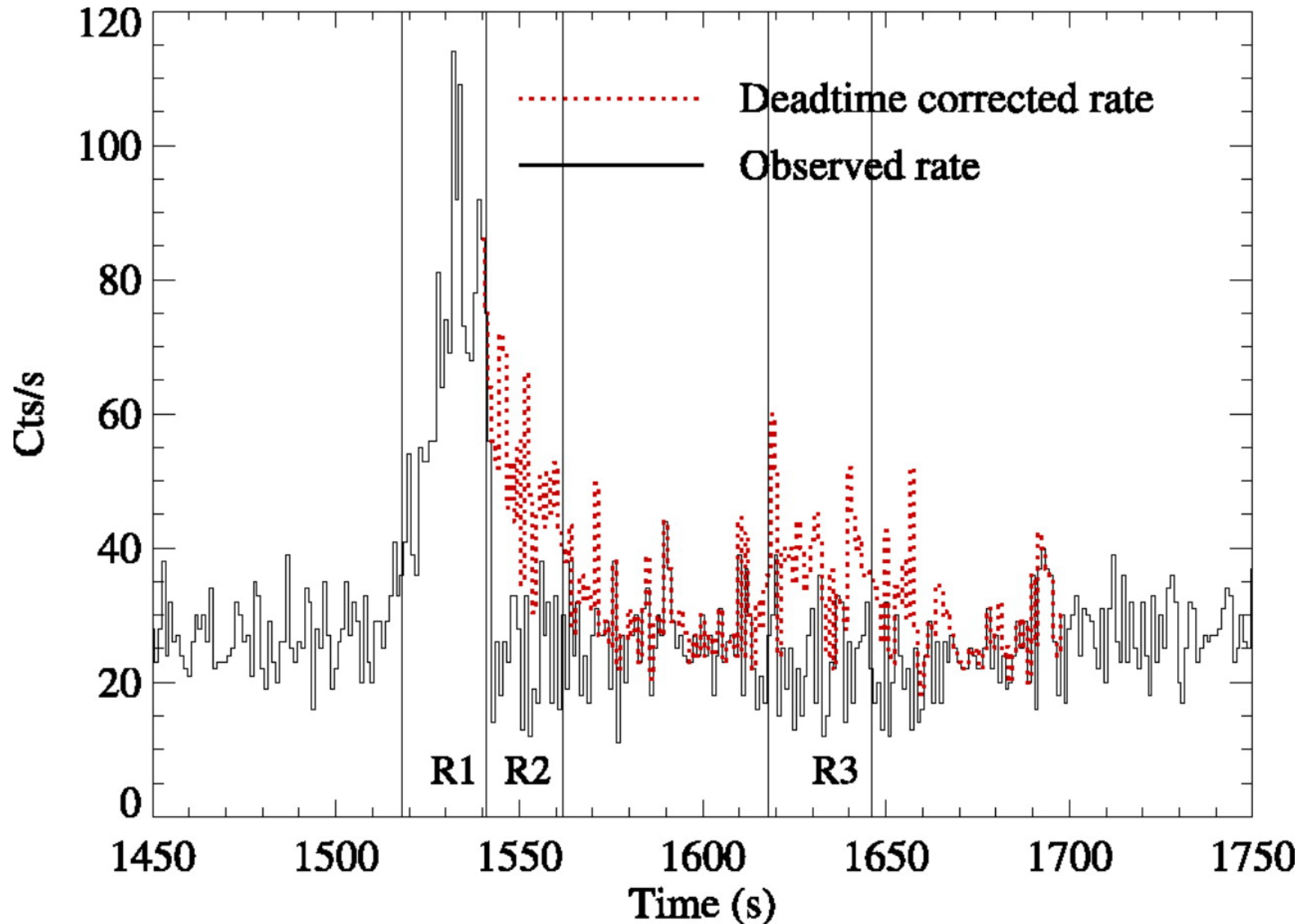
Fig. 3. from Search for Polarization from the Prompt GammaRay Emission of GRB 041219a with SPI on INTEGRAL Kalemci et al. 2007 ApJS 169 75 doi:10.1086/510676 https://dx.doi.org/10.1086/510676
