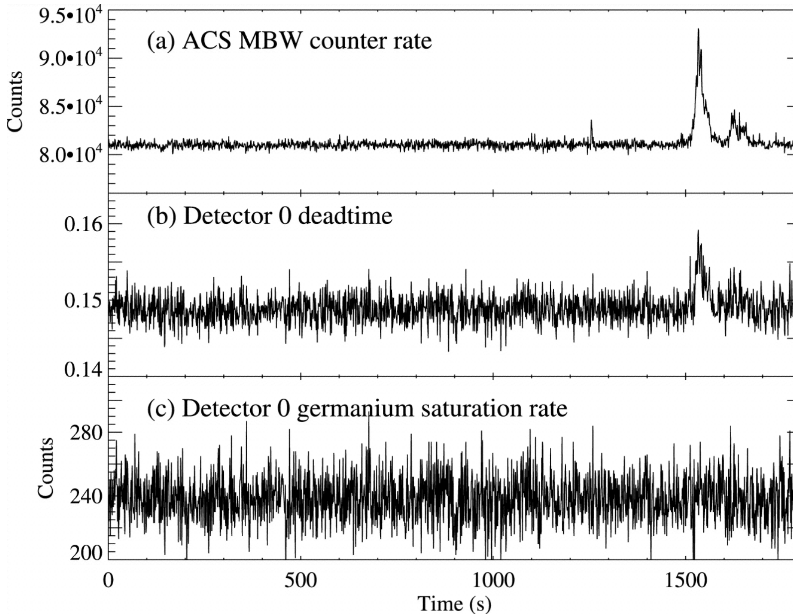
Fig. 2. from Search for Polarization from the Prompt GammaRay Emission of GRB 041219a with SPI on INTEGRAL Kalemci et al. 2007 ApJS 169 75 doi:10.1086/510676 https://dx.doi.org/10.1086/510676
