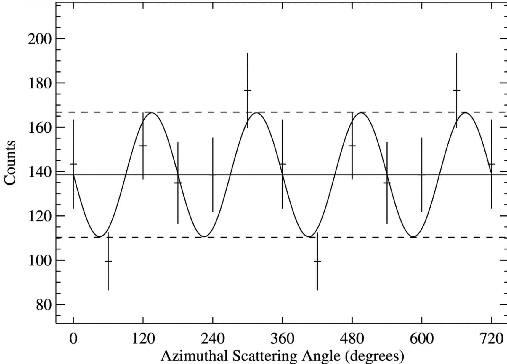
Fig. 11. from Search for Polarization from the Prompt GammaRay Emission of GRB 041219a with SPI on INTEGRAL Kalemci et al. 2007 ApJS 169 75 doi:10.1086/510676 https://dx.doi.org/10.1086/510676 © 2007. The American Astronomical Society. All rights reserved. Printed in U.S.A.
