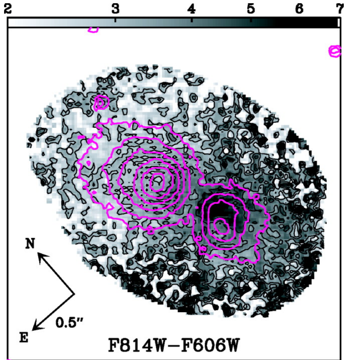
Fig. 8. from Adaptive Optics Imaging of IRAS 182761431: A Bipolar Preplanetary Nebula with Circumstellar “Searchlight Beams” and “Arcs” Sánchez Contreras et al. 2007 ApJ 656 1150 doi:10.1086/510480 https://dx.doi.org/10.1086/510480
