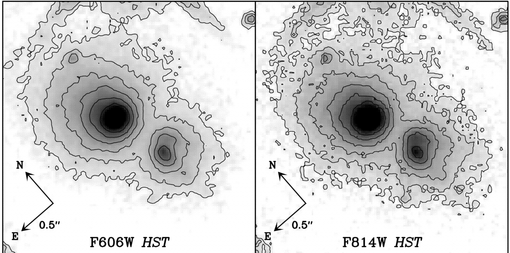
Fig. 4. from Adaptive Optics Imaging of IRAS 182761431: A Bipolar Preplanetary Nebula with Circumstellar “Searchlight Beams” and “Arcs” Sánchez Contreras et al. 2007 ApJ 656 1150 doi:10.1086/510480 https://dx.doi.org/10.1086/510480 © 2007. The American Astronomical Society. All rights reserved. Printed in U.S.A.
