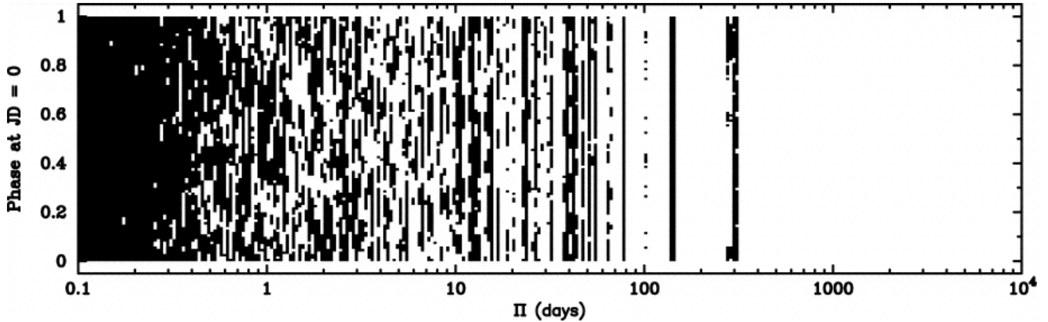
Fig. 13. from Asymmetry and Variability in the HH 30 Circumstellar Disk Watson & Stapelfeldt 2007 AJ 133 845 doi:10.1086/510455 https://dx.doi.org/10.1086/510455 © 2007. The American Astronomical Society. All rights reserved. Printed in U.S.A.
