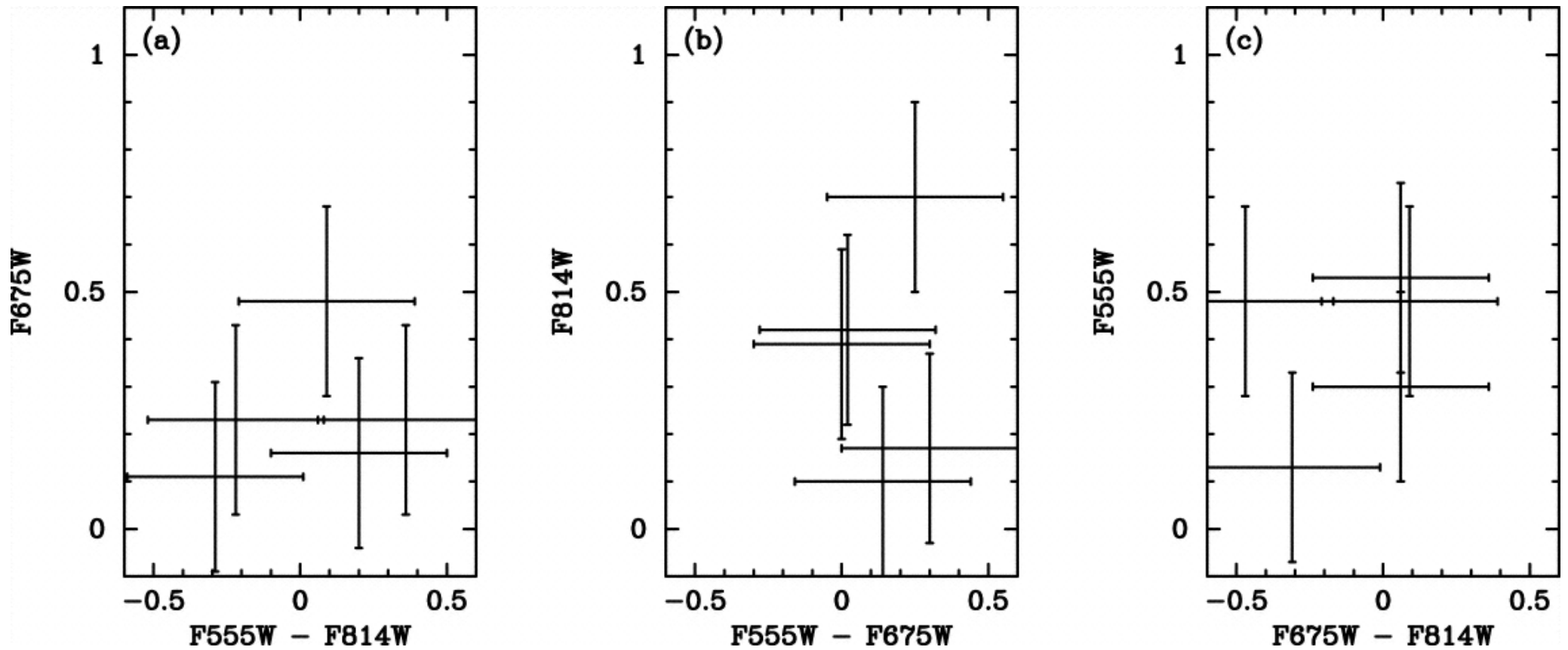
Fig. 10. from Asymmetry and Variability in the HH 30 Circumstellar Disk Watson & Stapelfeldt 2007 AJ 133 845 doi:10.1086/510455 https://dx.doi.org/10.1086/510455 © 2007. The American Astronomical Society. All rights reserved. Printed in U.S.A.
