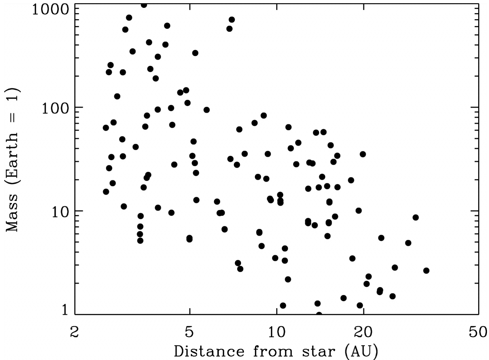
Fig. 4. from Planet Formation with Migration Chambers 2006 ApJL 652 L133 doi:10.1086/510407 https://dx.doi.org/10.1086/510407
