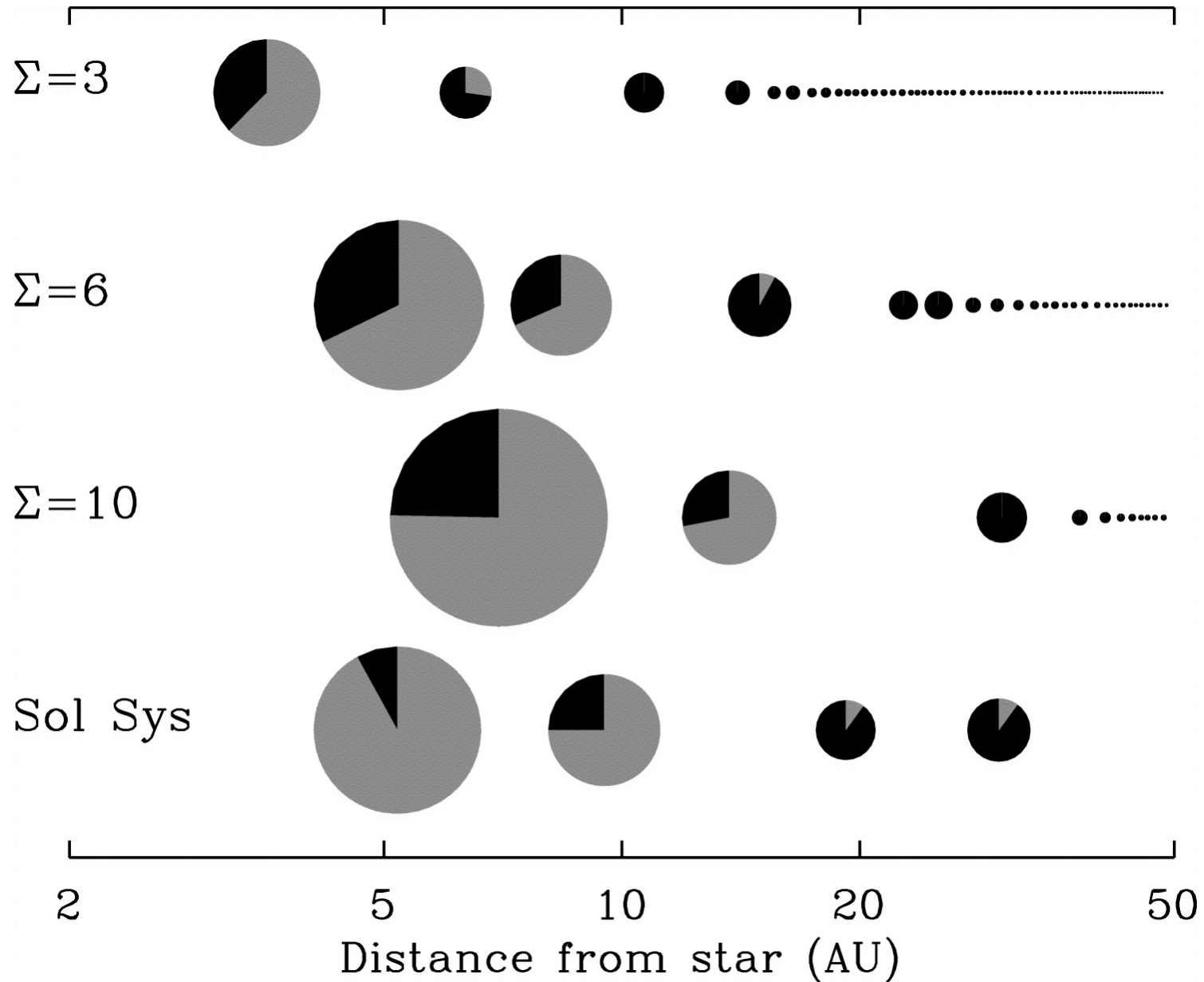
Fig. 3. from Planet Formation with Migration Chambers 2006 ApJL 652 L133 doi:10.1086/510407 https://dx.doi.org/10.1086/510407
