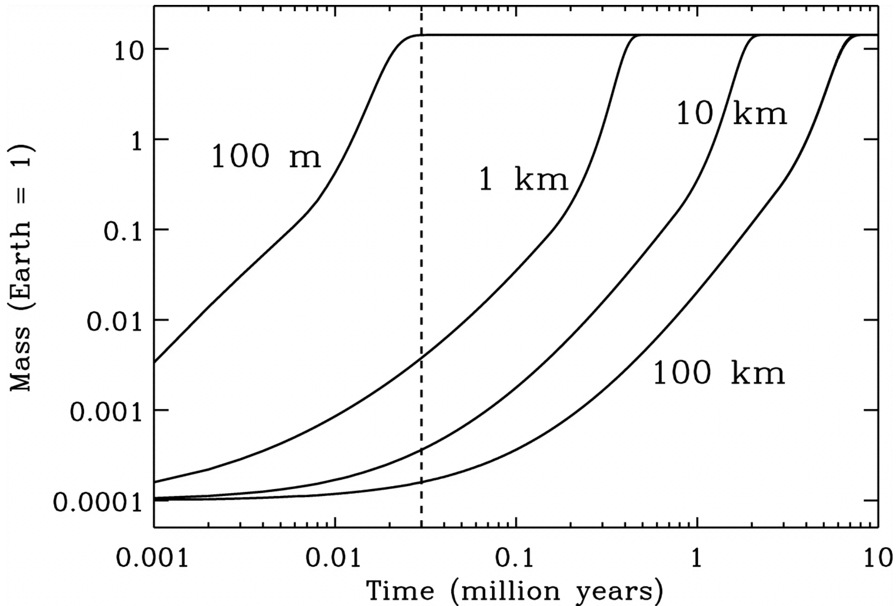
Fig. 1. from Planet Formation with Migration Chambers 2006 ApJL 652 L133 doi:10.1086/510407 https://dx.doi.org/10.1086/510407
