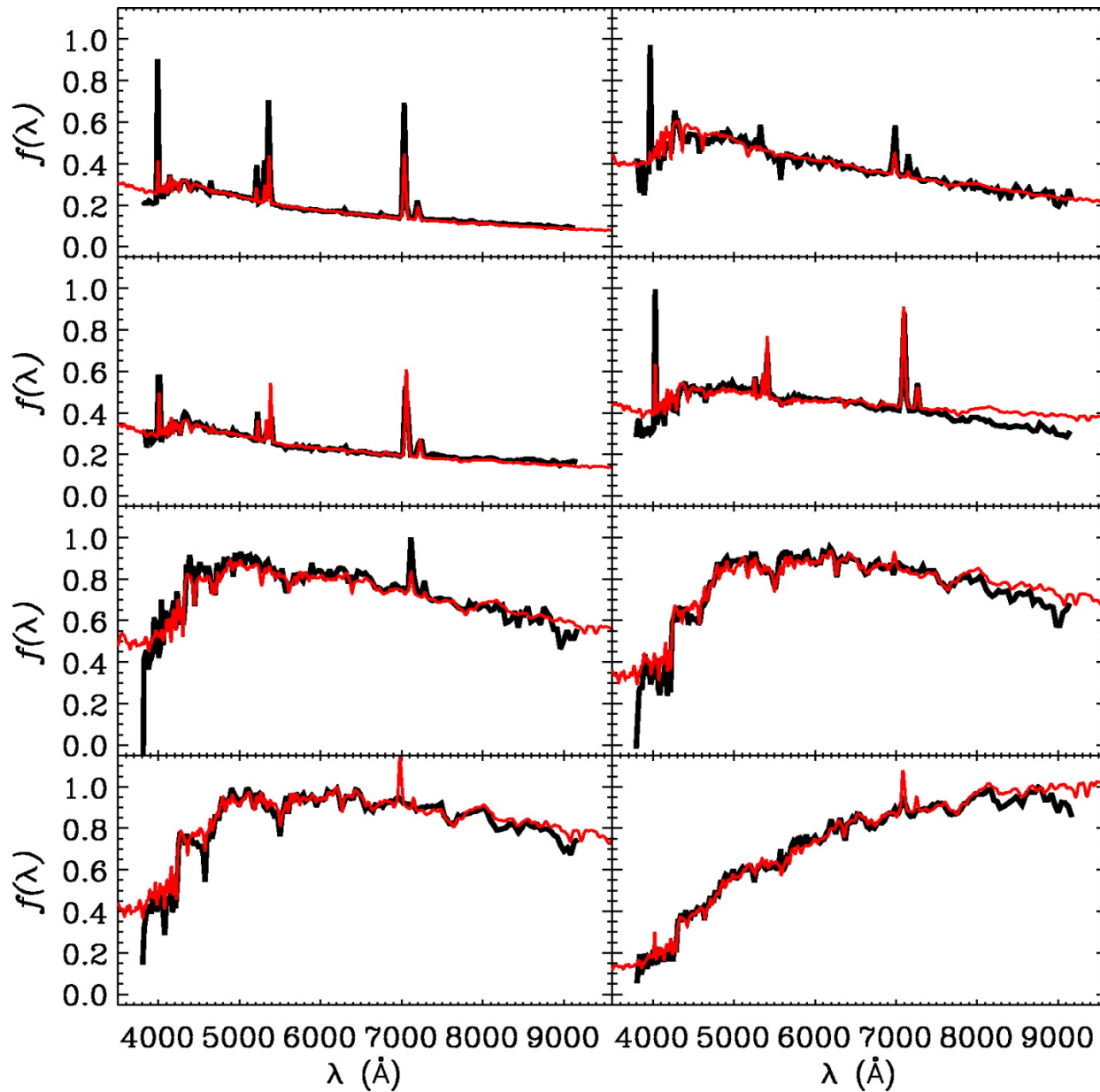
Fig. 8. from KCorrections and Filter Transformations in the Ultraviolet, Optical, and NearInfrared Blanton & Roweis 2007 AJ 133 734 doi:10.1086/510127 https://dx.doi.org/10.1086/510127
