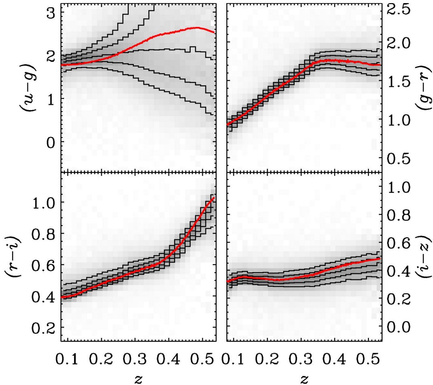
Fig. 3. from KCorrections and Filter Transformations in the Ultraviolet, Optical, and NearInfrared Blanton & Roweis 2007 AJ 133 734 doi:10.1086/510127 https://dx.doi.org/10.1086/510127
