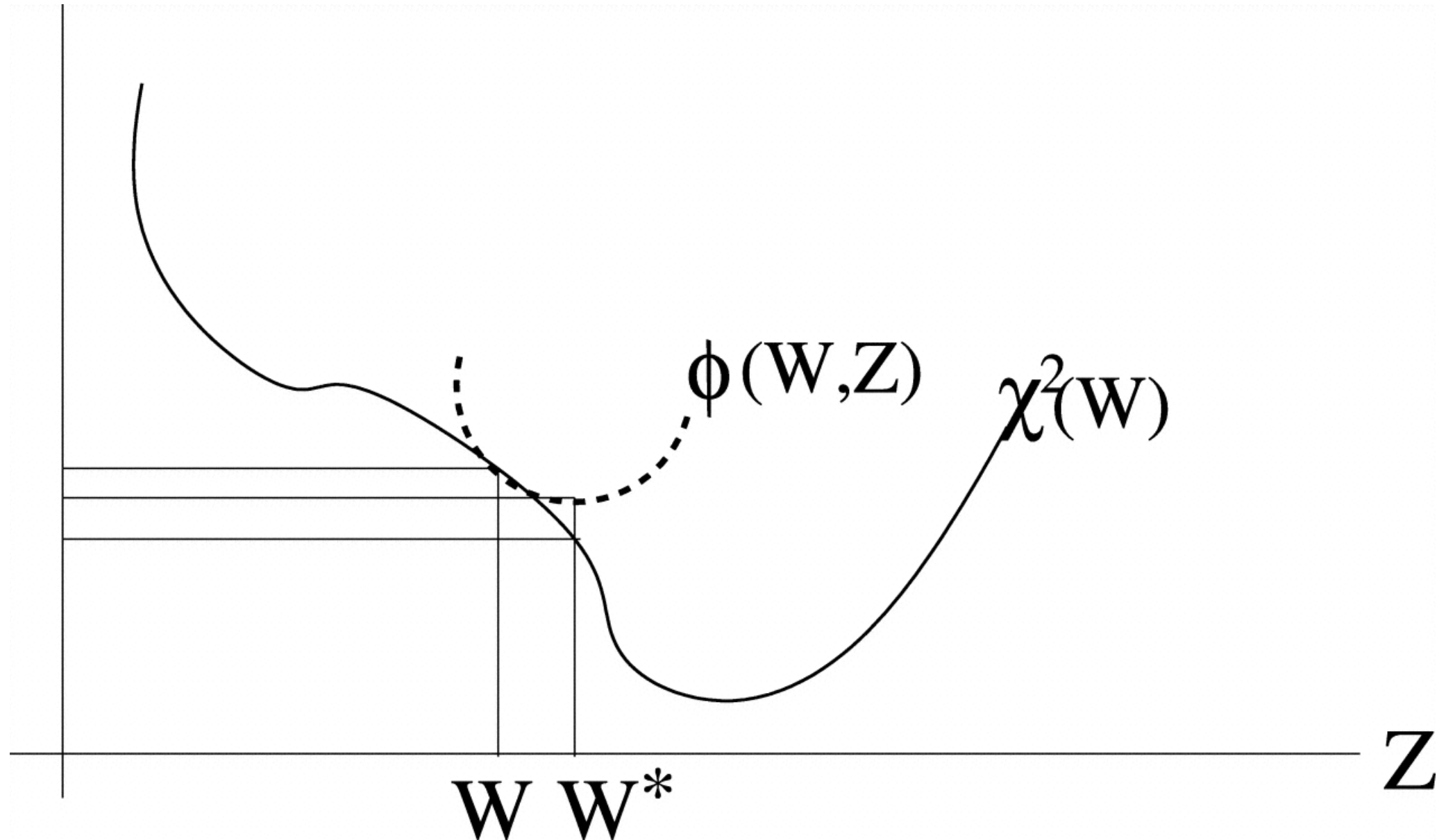
Fig. 20. from KCorrections and Filter Transformations in the Ultraviolet, Optical, and NearInfrared Blanton & Roweis 2007 AJ 133 734 doi:10.1086/510127 https://dx.doi.org/10.1086/510127 © 2007. The American Astronomical Society. All rights reserved. Printed in U.S.A.
