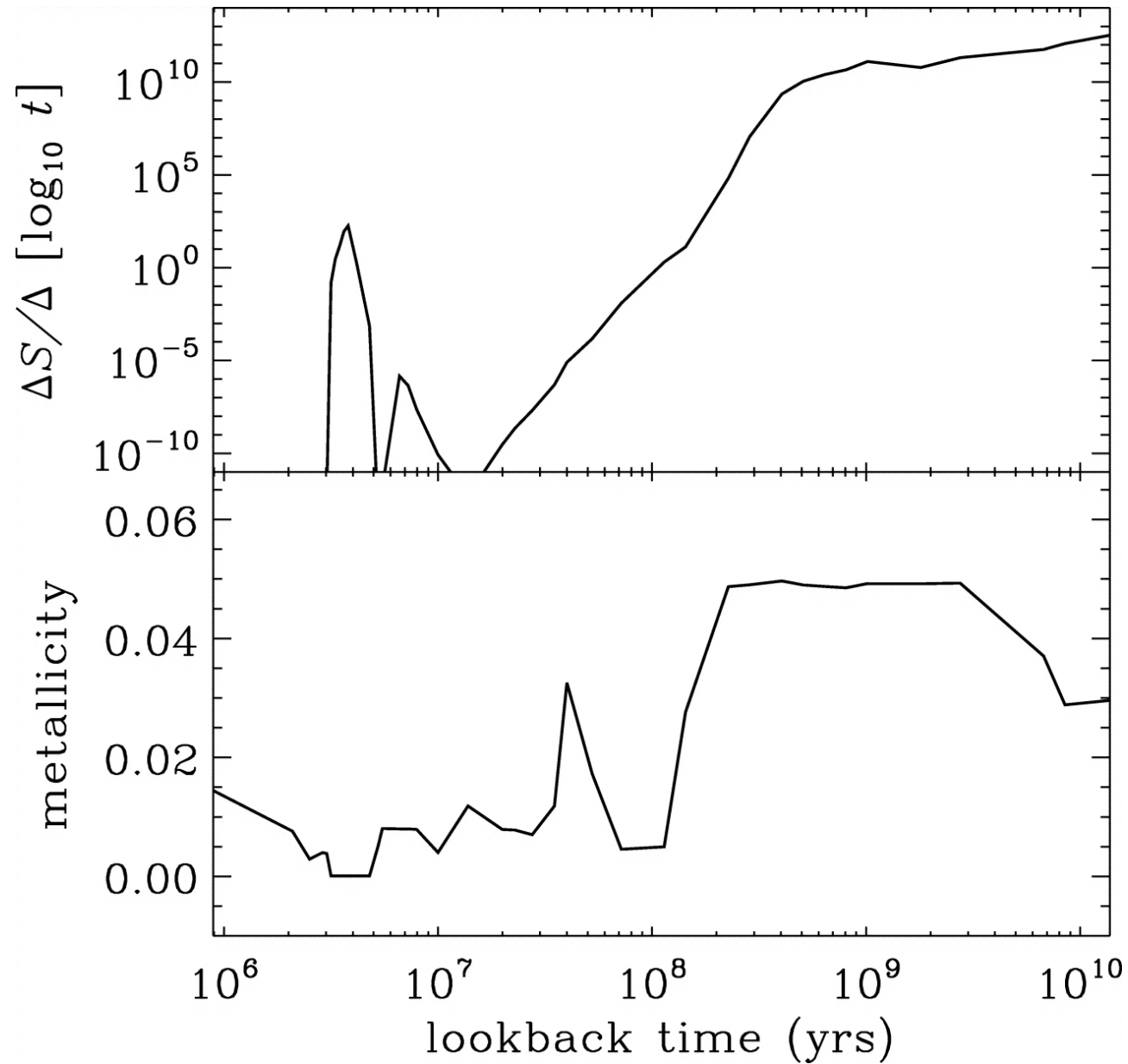
Fig. 2. from KCorrections and Filter Transformations in the Ultraviolet, Optical, and NearInfrared Blanton & Roweis 2007 AJ 133 734 doi:10.1086/510127 https://dx.doi.org/10.1086/510127 © 2007. The American Astronomical Society. All rights reserved. Printed in U.S.A.
