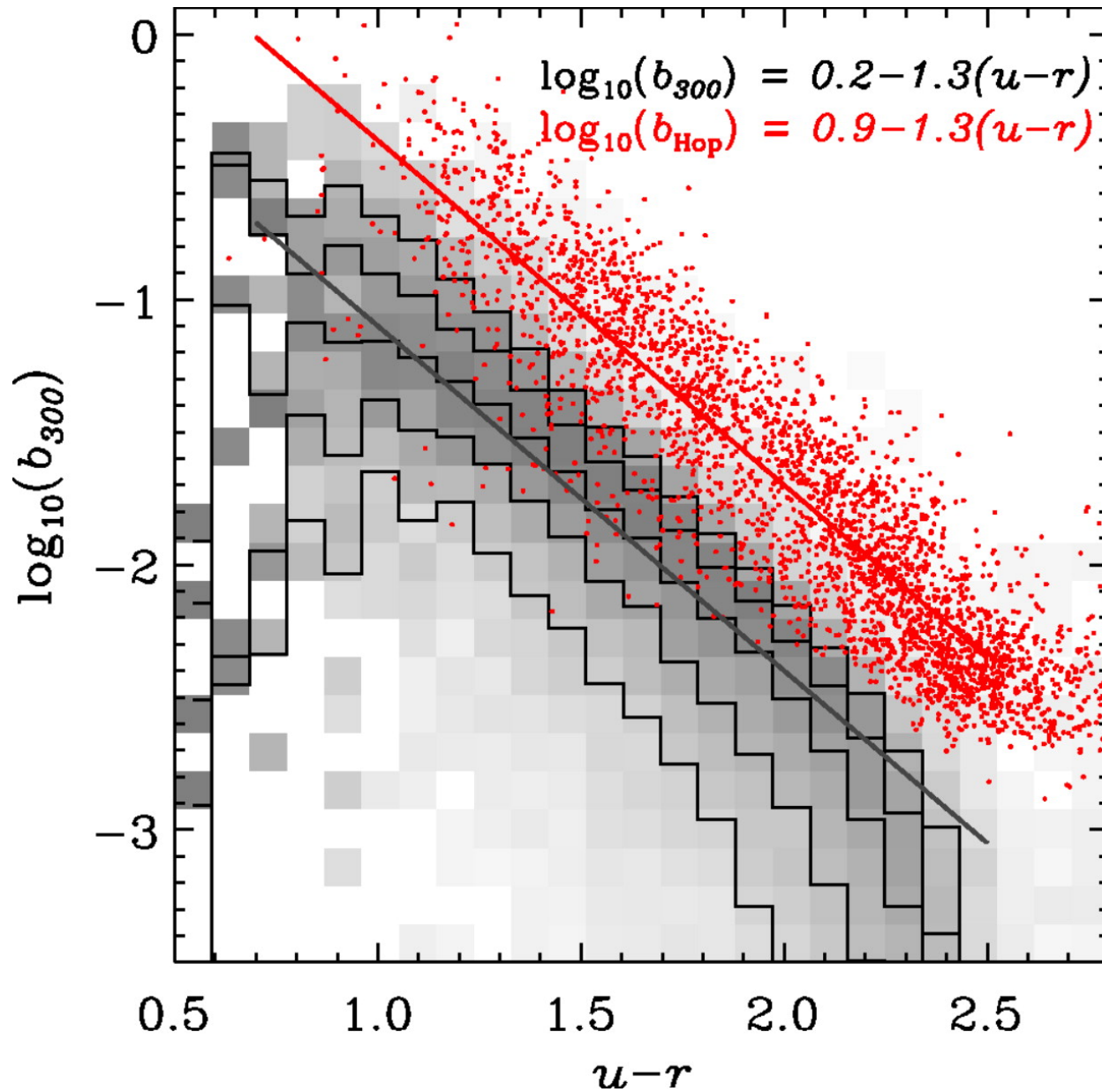
Fig. 19. from KCorrections and Filter Transformations in the Ultraviolet, Optical, and NearInfrared Blanton & Roweis 2007 AJ 133 734 doi:10.1086/510127 https://dx.doi.org/10.1086/510127 © 2007. The American Astronomical Society. All rights reserved. Printed in U.S.A.
