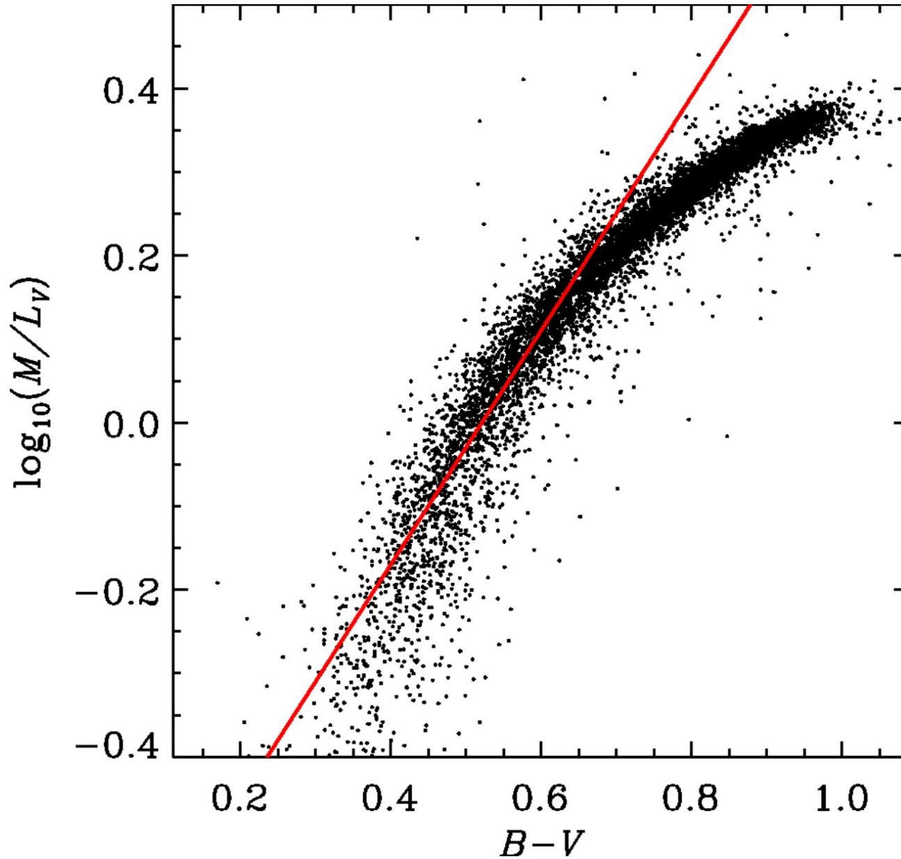
Fig. 18. from KCorrections and Filter Transformations in the Ultraviolet, Optical, and NearInfrared Blanton & Roweis 2007 AJ 133 734 doi:10.1086/510127 https://dx.doi.org/10.1086/510127 © 2007. The American Astronomical Society. All rights reserved. Printed in U.S.A.
