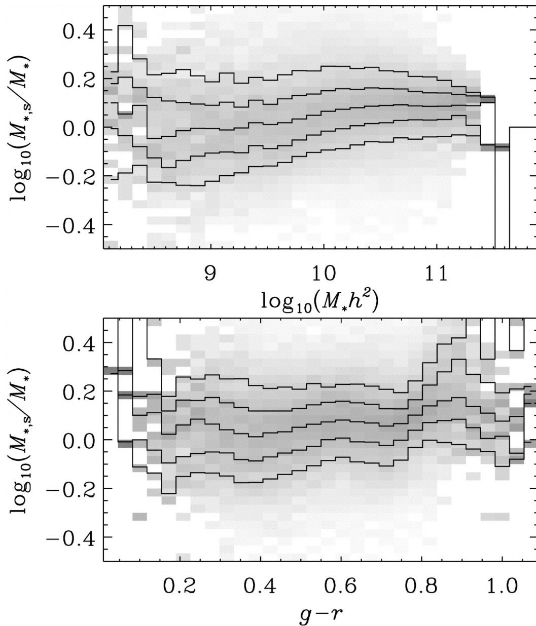
Fig. 17. from KCorrections and Filter Transformations in the Ultraviolet, Optical, and NearInfrared Blanton & Roweis 2007 AJ 133 734 doi:10.1086/510127 https://dx.doi.org/10.1086/510127
