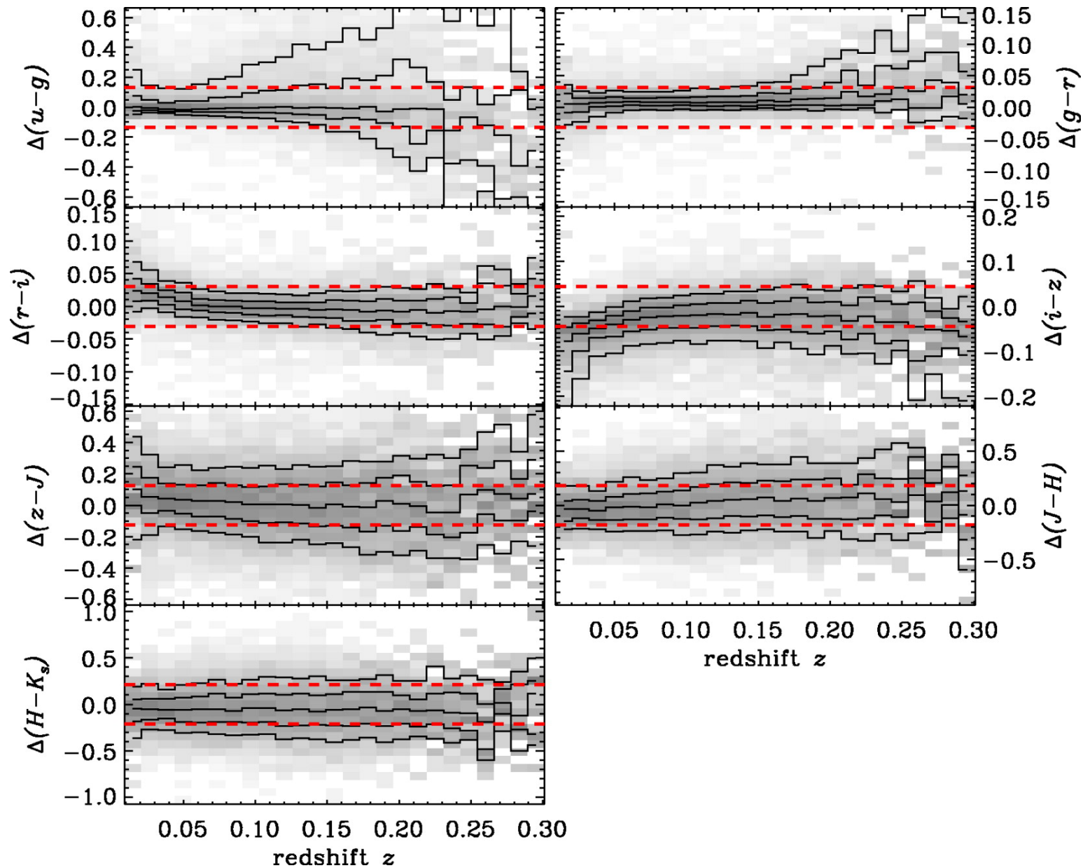
Fig. 10. from KCorrections and Filter Transformations in the Ultraviolet, Optical, and NearInfrared Blanton & Roweis 2007 AJ 133 734 doi:10.1086/510127 https://dx.doi.org/10.1086/510127
