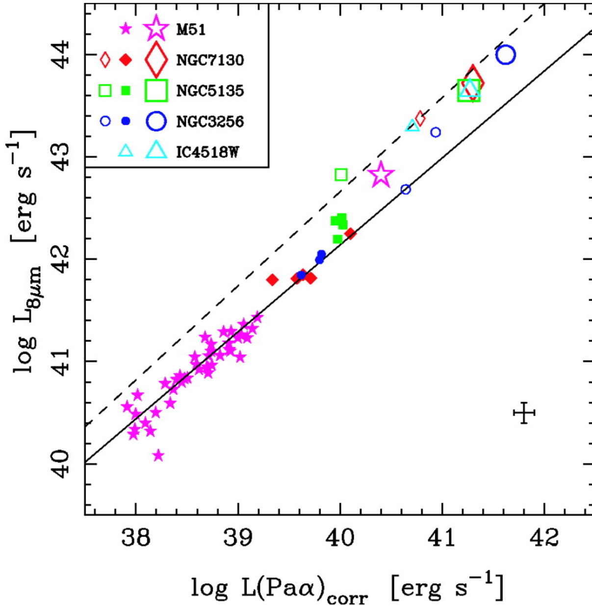
Fig. 3. from High Spatial Resolution TReCS MidInfrared Imaging of Luminous Infrared Galaxies AlonsoHerrero et al. 2006 ApJL 652 L83 doi:10.1086/510016 https://dx.doi.org/10.1086/510016 © 2006. The American Astronomical Society. All rights reserved. Printed in U.S.A.
