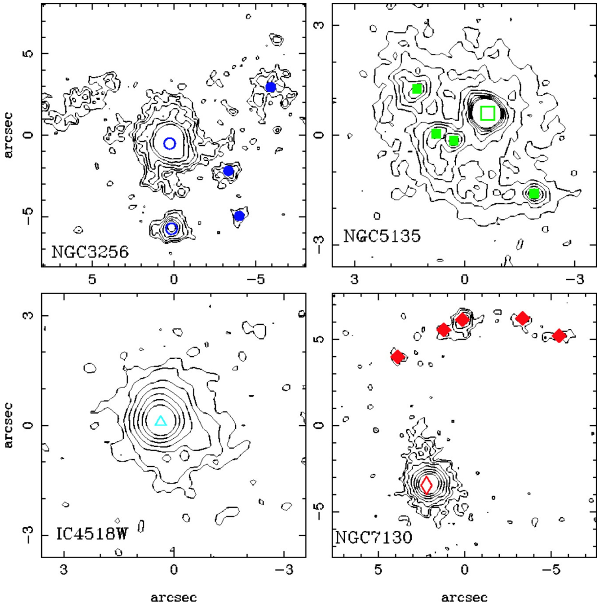
Fig. 2. from High Spatial Resolution TReCS MidInfrared Imaging of Luminous Infrared Galaxies AlonsoHerrero et al. 2006 ApJL 652 L83 doi:10.1086/510016 https://dx.doi.org/10.1086/510016 © 2006. The American Astronomical Society. All rights reserved. Printed in U.S.A.
