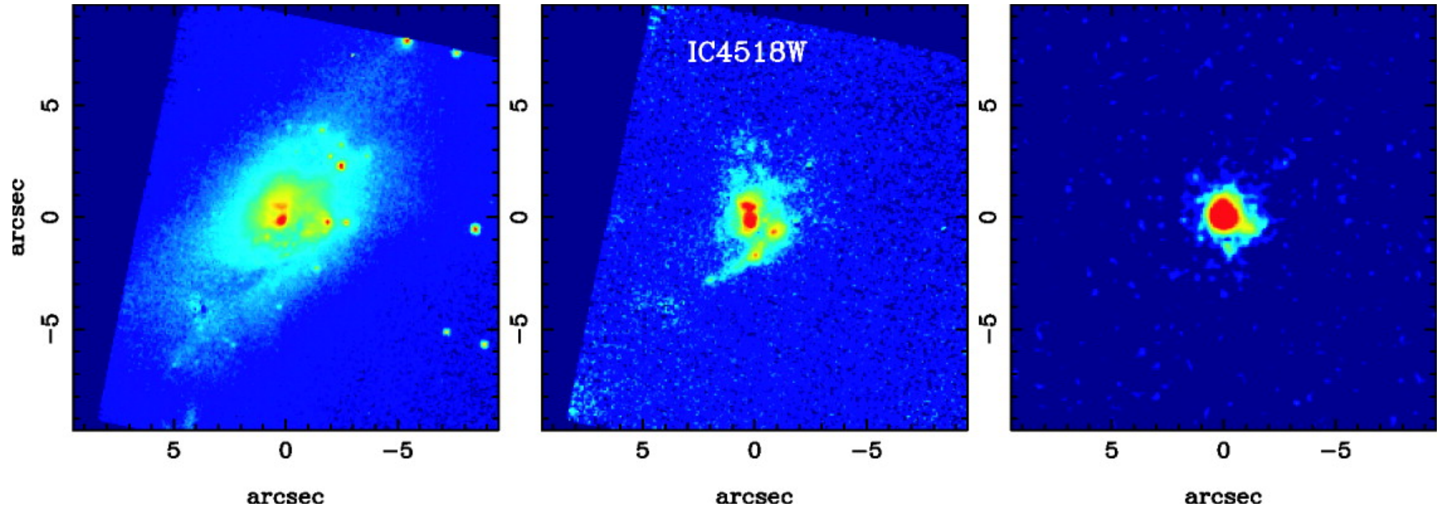
Fig. 1. from High Spatial Resolution TReCS MidInfrared Imaging of Luminous Infrared Galaxies AlonsoHerrero et al. 2006 ApJL 652 L83 doi:10.1086/510016 https://dx.doi.org/10.1086/510016
