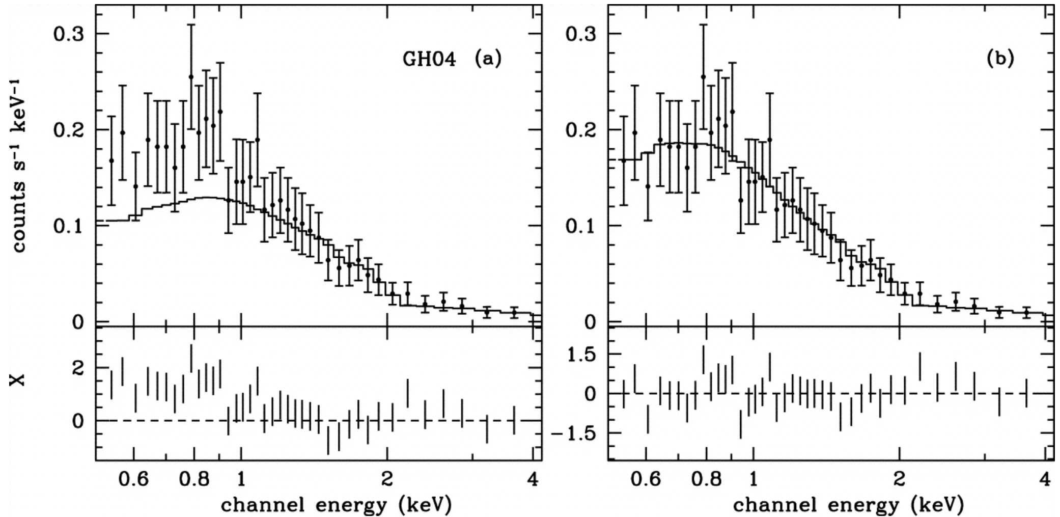
Fig. 2. from XRay Properties of IntermediateMass Black Holes in Active Galaxies Greene & Ho 2007 ApJ 656 84 doi:10.1086/509064 https://dx.doi.org/10.1086/509064 © 2007. The American Astronomical Society. All rights reserved. Printed in U.S.A.
