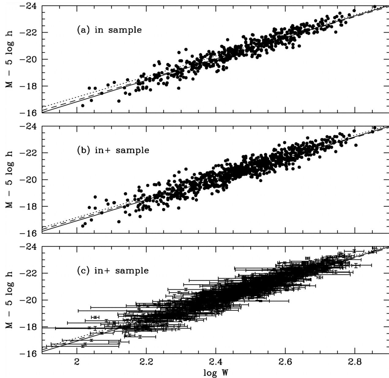
Fig. 9. from SFI++ I: A New IBand TullyFisher Template, the Cluster Peculiar Velocity Dispersion, and H0 Masters et al. 2006 ApJ 653 861 doi:10.1086/508924 https://dx.doi.org/10.1086/508924
