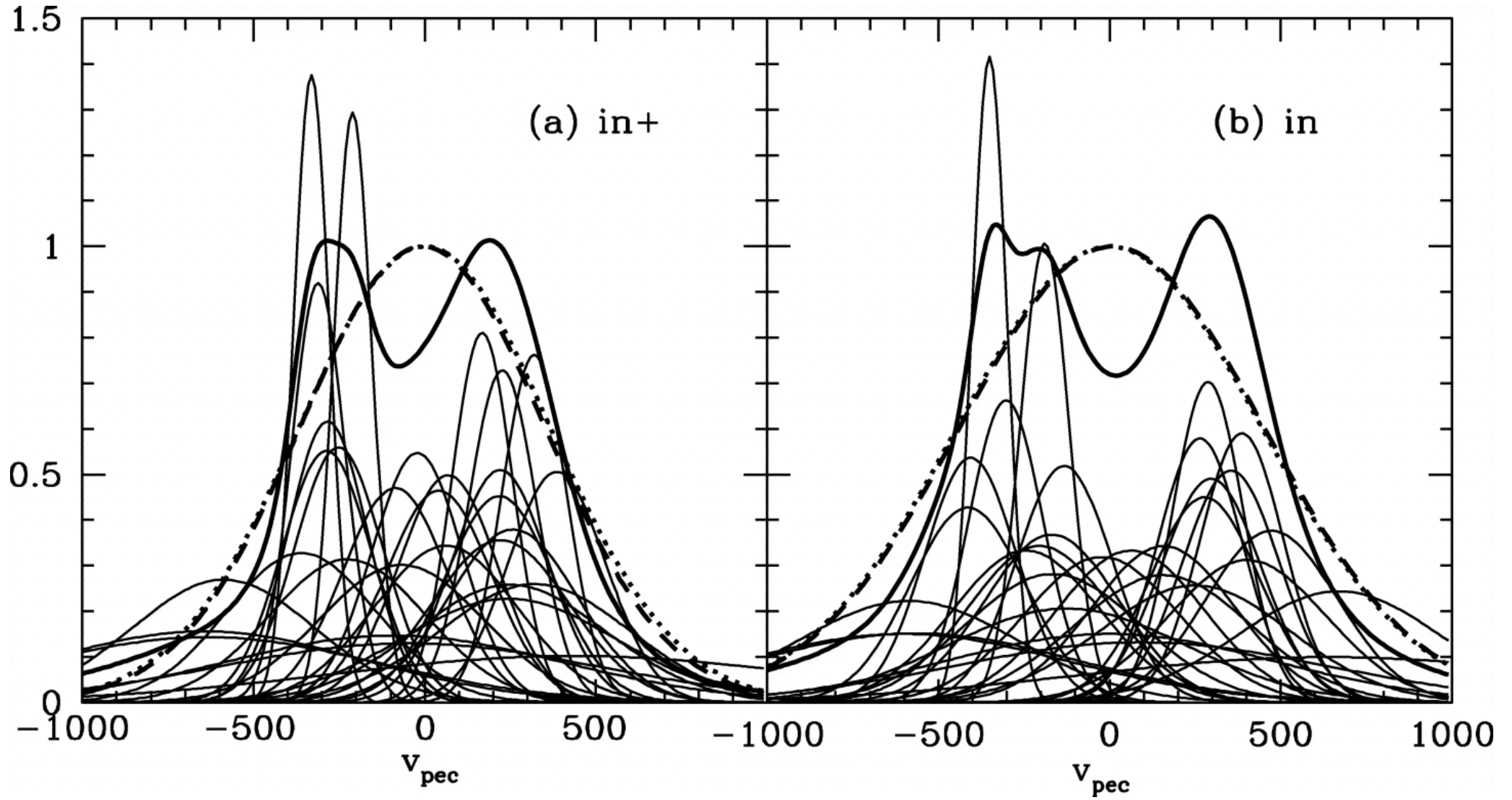
Fig. 8. from SFI++ I: A New IBand TullyFisher Template, the Cluster Peculiar Velocity Dispersion, and H0 Masters et al. 2006 ApJ 653 861 doi:10.1086/508924 https://dx.doi.org/10.1086/508924
