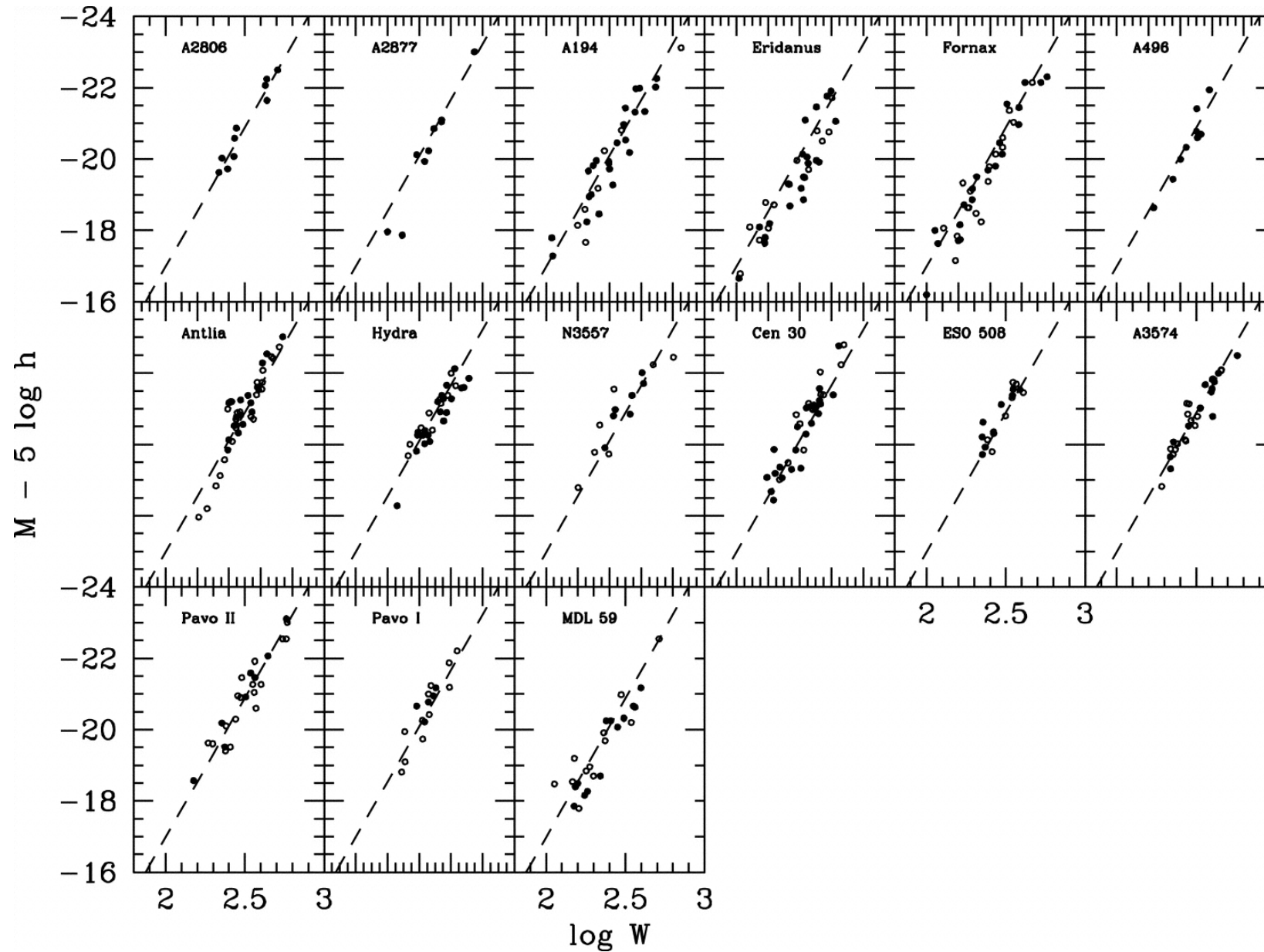
Fig. 6. from SFI++ I: A New IBand TullyFisher Template, the Cluster Peculiar Velocity Dispersion, and H0 Masters et al. 2006 ApJ 653 861 doi:10.1086/508924 https://dx.doi.org/10.1086/508924
