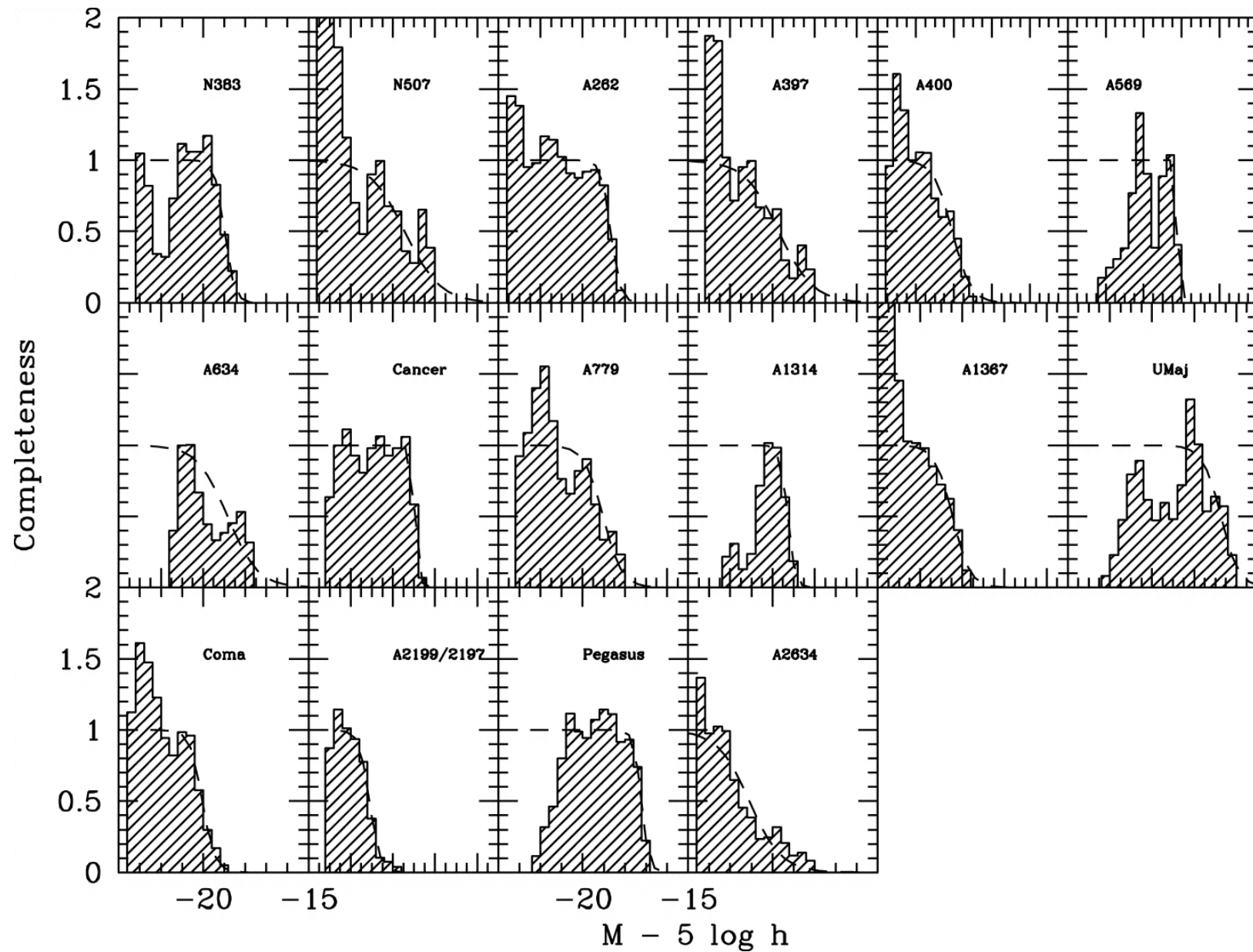
Fig. 3. from SFI++ I: A New IBand TullyFisher Template, the Cluster Peculiar Velocity Dispersion, and H0 Masters et al. 2006 ApJ 653 861 doi:10.1086/508924 https://dx.doi.org/10.1086/508924
