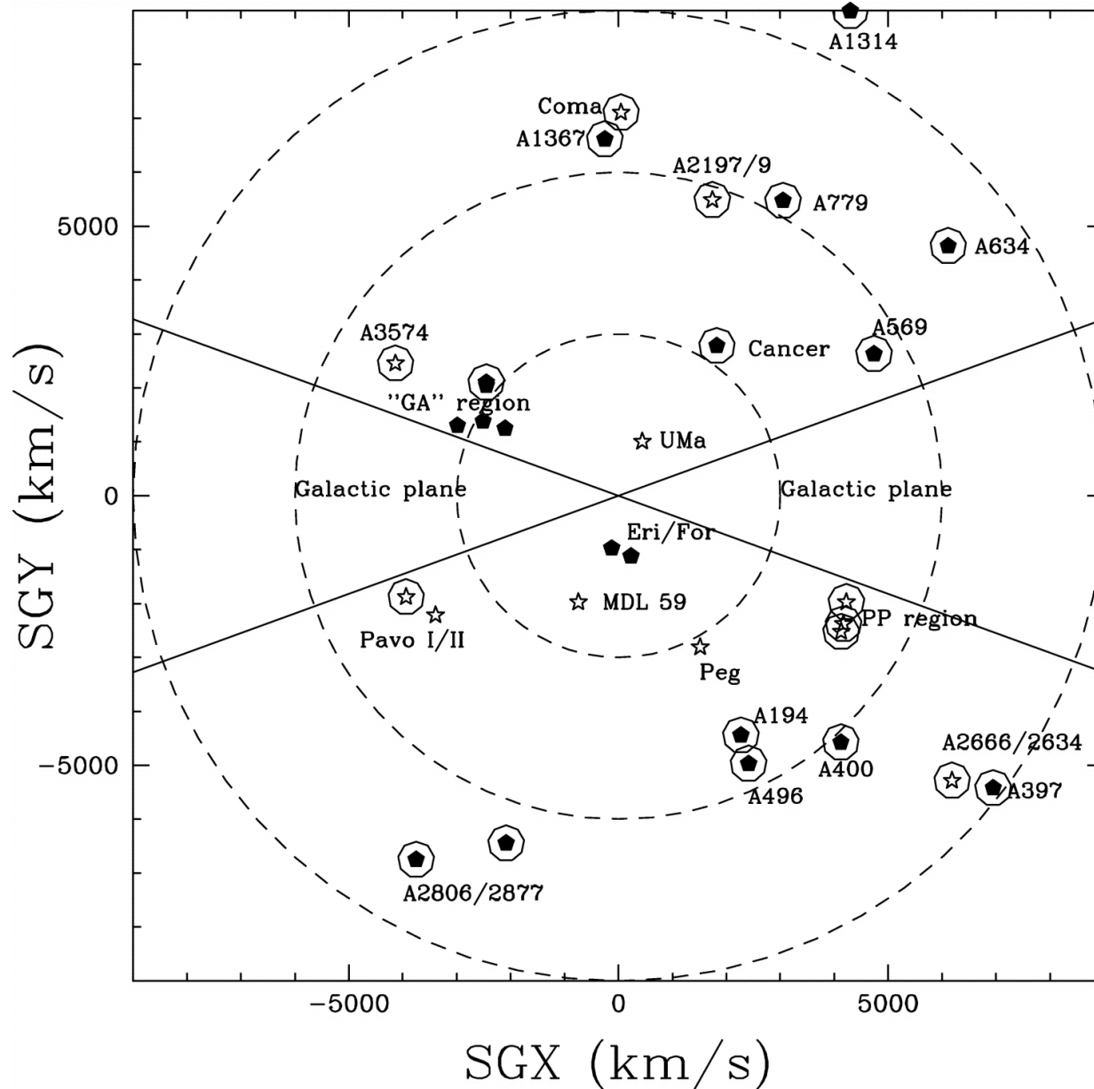
Fig. 2. from SFI++ I: A New IBand TullyFisher Template, the Cluster Peculiar Velocity Dispersion, and H0 Masters et al. 2006 ApJ 653 861 doi:10.1086/508924 https://dx.doi.org/10.1086/508924 © 2006. The American Astronomical Society. All rights reserved. Printed in U.S.A.
