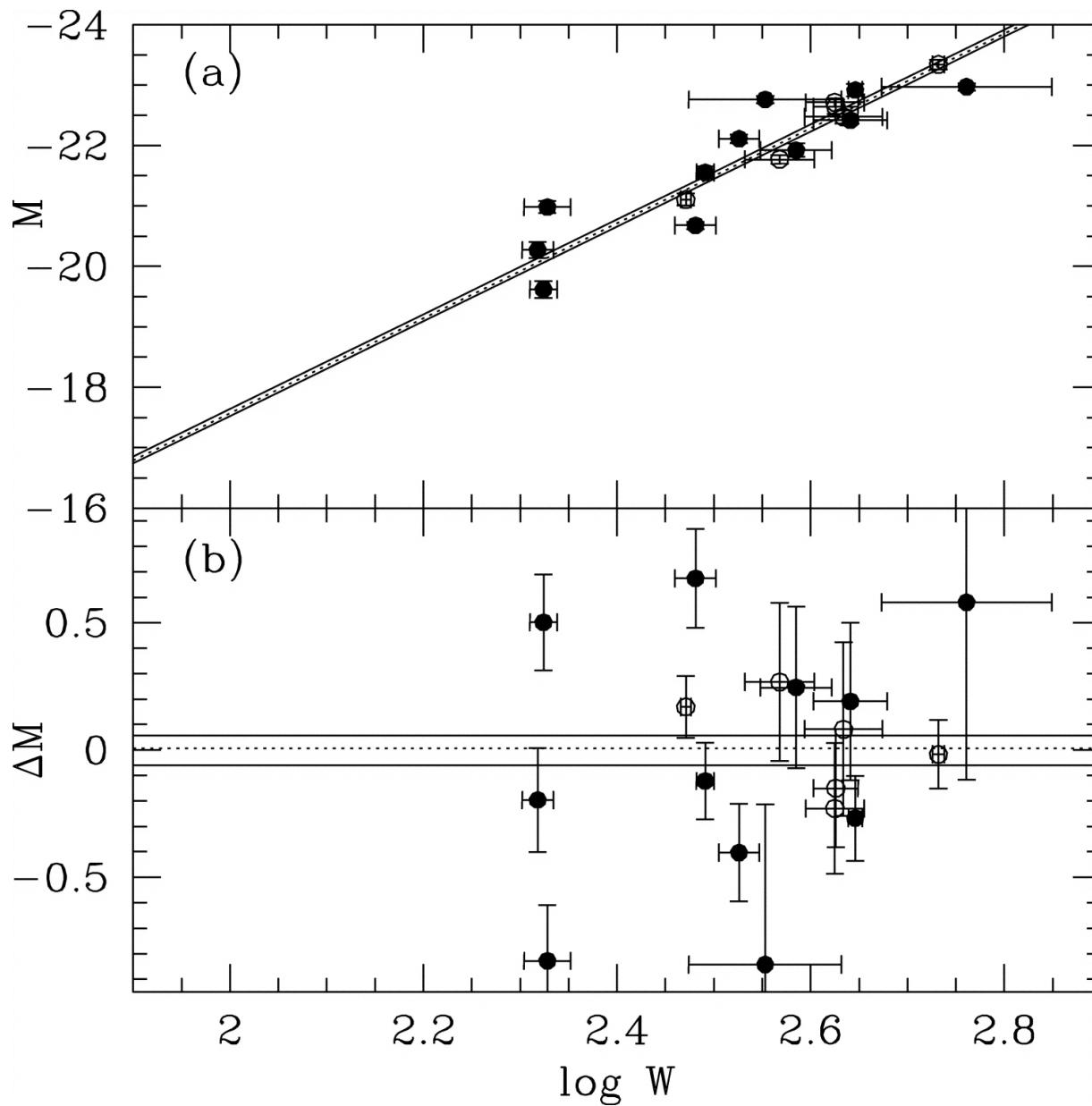
Fig. 12. from SFI++ I: A New IBand TullyFisher Template, the Cluster Peculiar Velocity Dispersion, and H0 Masters et al. 2006 ApJ 653 861 doi:10.1086/508924 https://dx.doi.org/10.1086/508924
