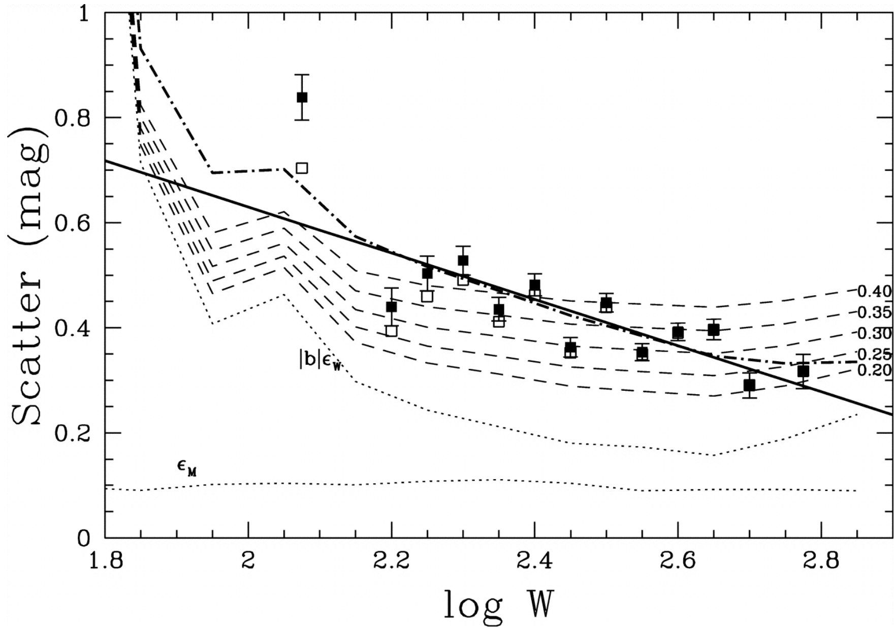
Fig. 11. from SFI++ I: A New IBand TullyFisher Template, the Cluster Peculiar Velocity Dispersion, and H0 Masters et al. 2006 ApJ 653 861 doi:10.1086/508924 https://dx.doi.org/10.1086/508924 © 2006. The American Astronomical Society. All rights reserved. Printed in U.S.A.
