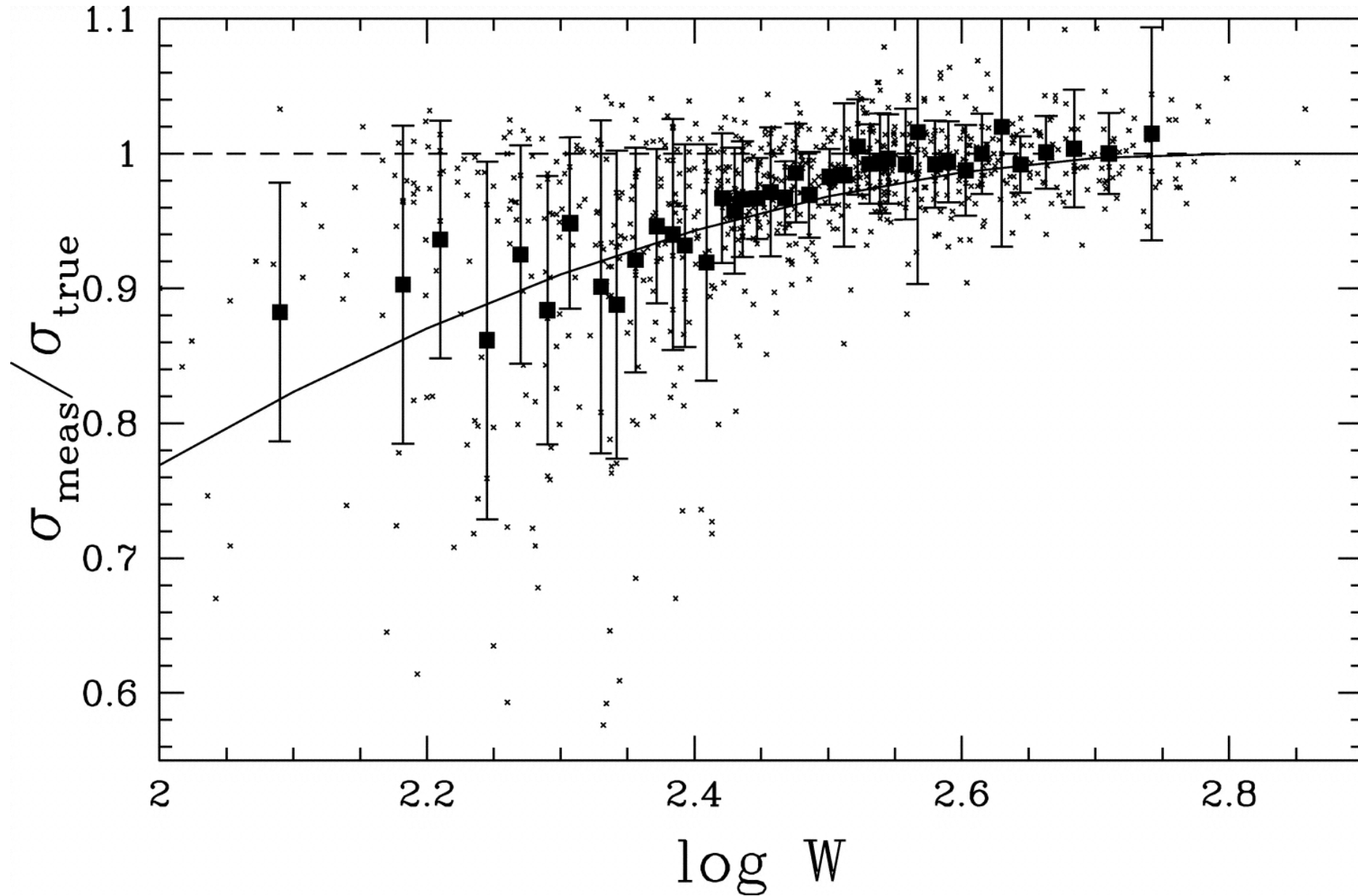
Fig. 10. from SFI++ I: A New IBand TullyFisher Template, the Cluster Peculiar Velocity Dispersion, and H0 Masters et al. 2006 ApJ 653 861 doi:10.1086/508924 https://dx.doi.org/10.1086/508924
