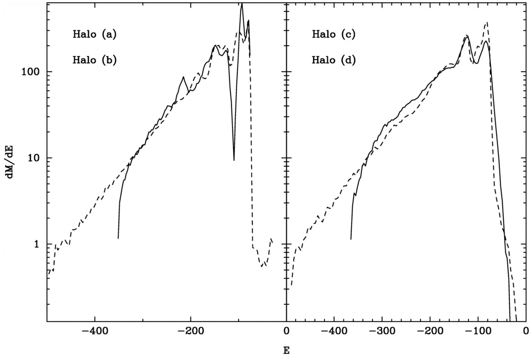
Fig. 9. from On Universal Halos and the Radial Orbit Instability MacMillan, Widrow, & Henriksen 2006 ApJ 653 43 doi:10.1086/508602 https://dx.doi.org/10.1086/508602
