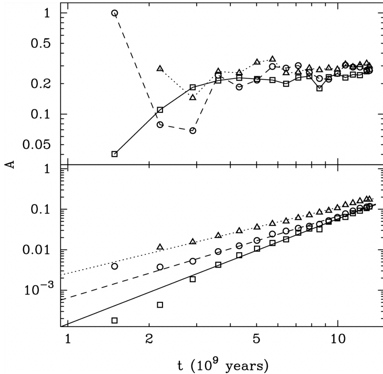
Fig. 8. from On Universal Halos and the Radial Orbit Instability MacMillan, Widrow, & Henriksen 2006 ApJ 653 43 doi:10.1086/508602 https://dx.doi.org/10.1086/508602
