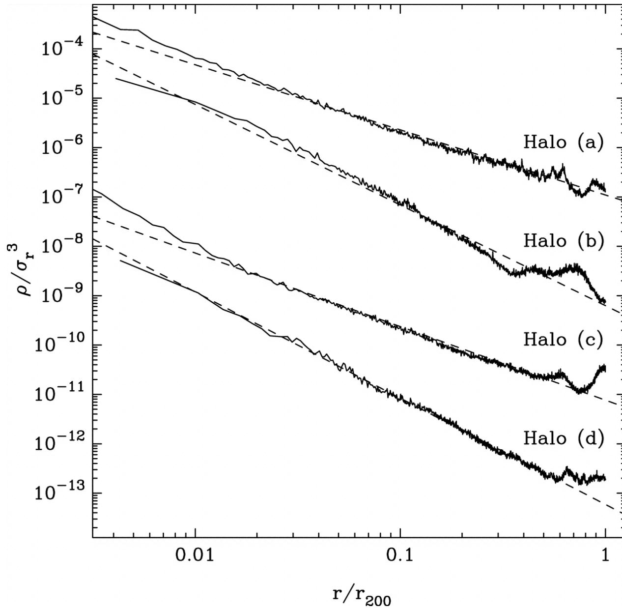
Fig. 7. from On Universal Halos and the Radial Orbit Instability MacMillan, Widrow, & Henriksen 2006 ApJ 653 43 doi:10.1086/508602 https://dx.doi.org/10.1086/508602
