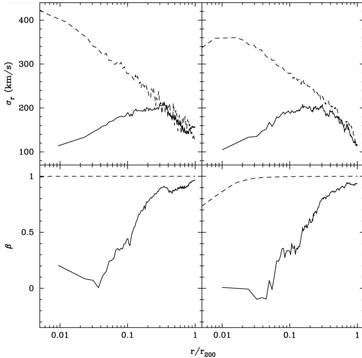
Fig. 6. from On Universal Halos and the Radial Orbit Instability MacMillan, Widrow, & Henriksen 2006 ApJ 653 43 doi:10.1086/508602 https://dx.doi.org/10.1086/508602
