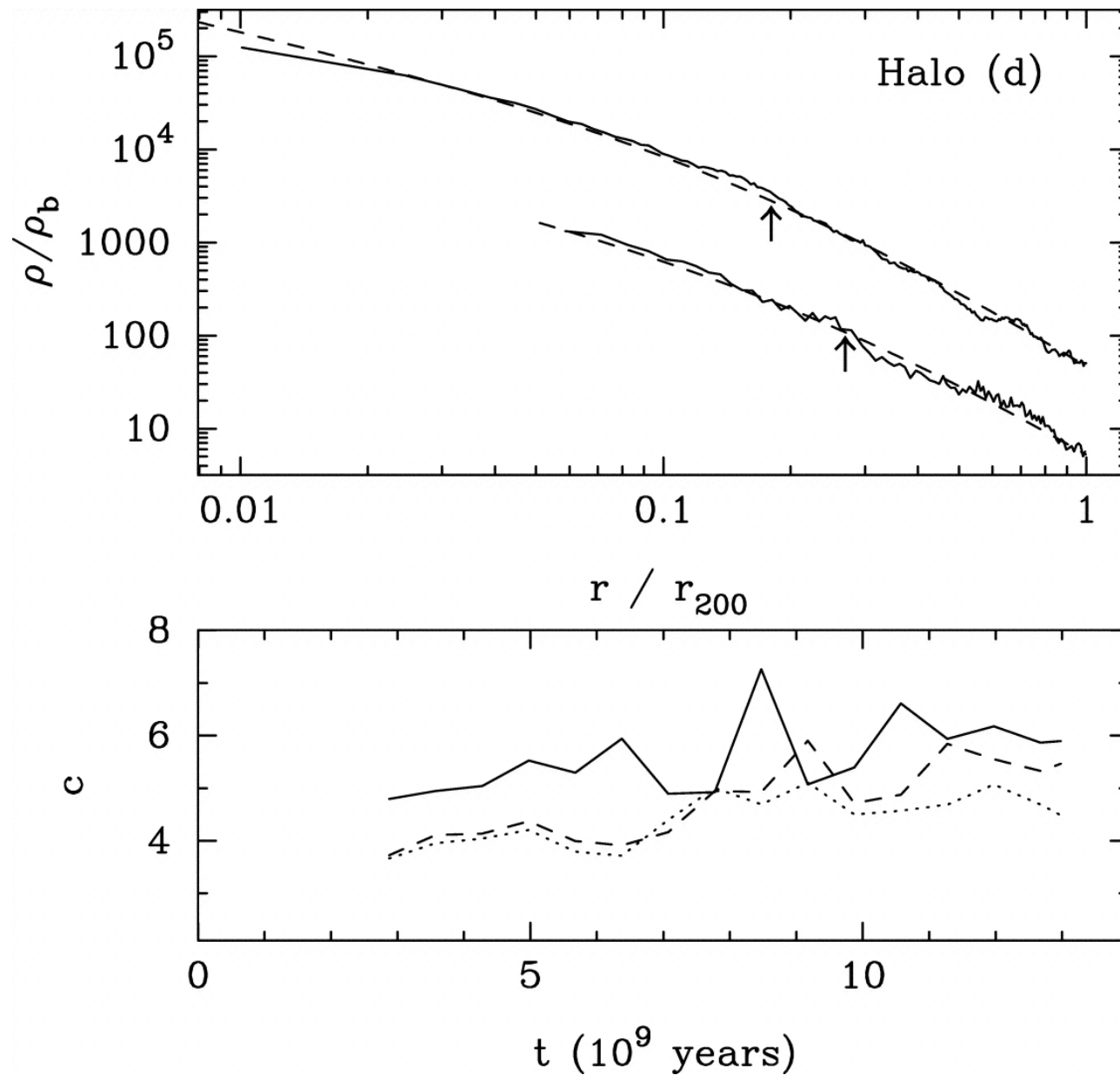
Fig. 4. from On Universal Halos and the Radial Orbit Instability MacMillan, Widrow, & Henriksen 2006 ApJ 653 43 doi:10.1086/508602 https://dx.doi.org/10.1086/508602
