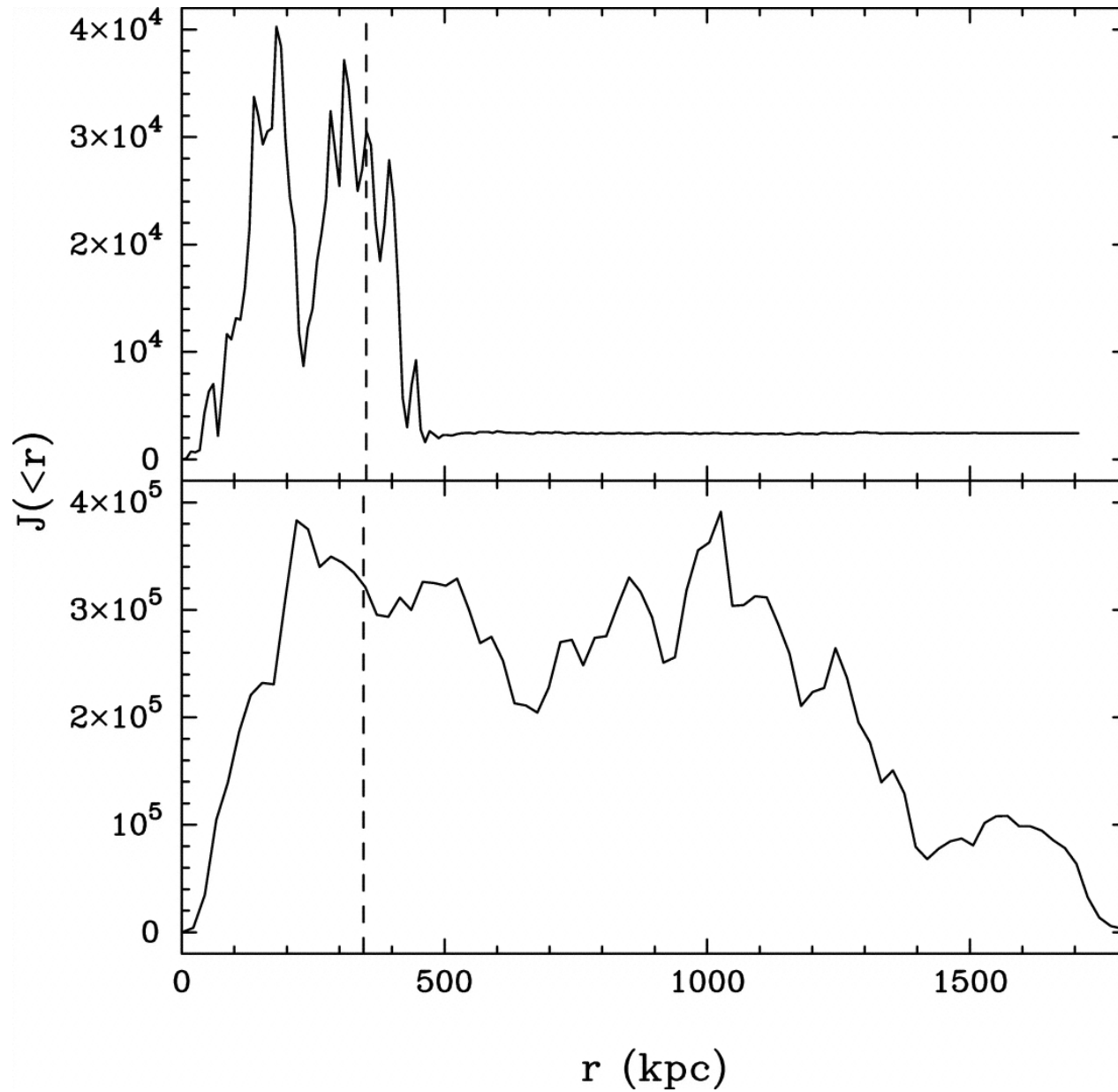
Fig. 2. from On Universal Halos and the Radial Orbit Instability MacMillan, Widrow, & Henriksen 2006 ApJ 653 43 doi:10.1086/508602 https://dx.doi.org/10.1086/508602
