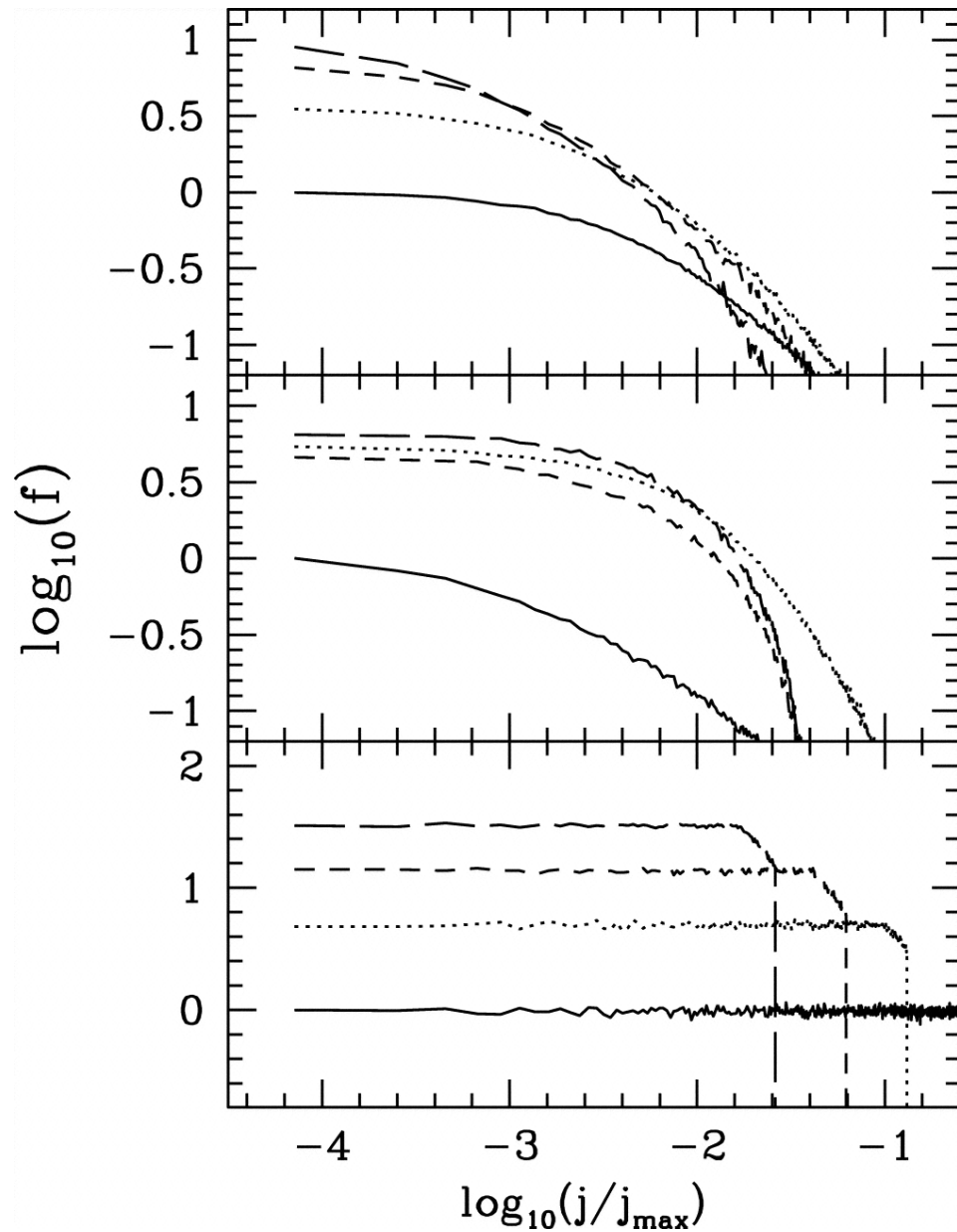
Fig. 12. from On Universal Halos and the Radial Orbit Instability MacMillan, Widrow, & Henriksen 2006 ApJ 653 43 doi:10.1086/508602 https://dx.doi.org/10.1086/508602 © 2006. The American Astronomical Society. All rights reserved. Printed in U.S.A.
