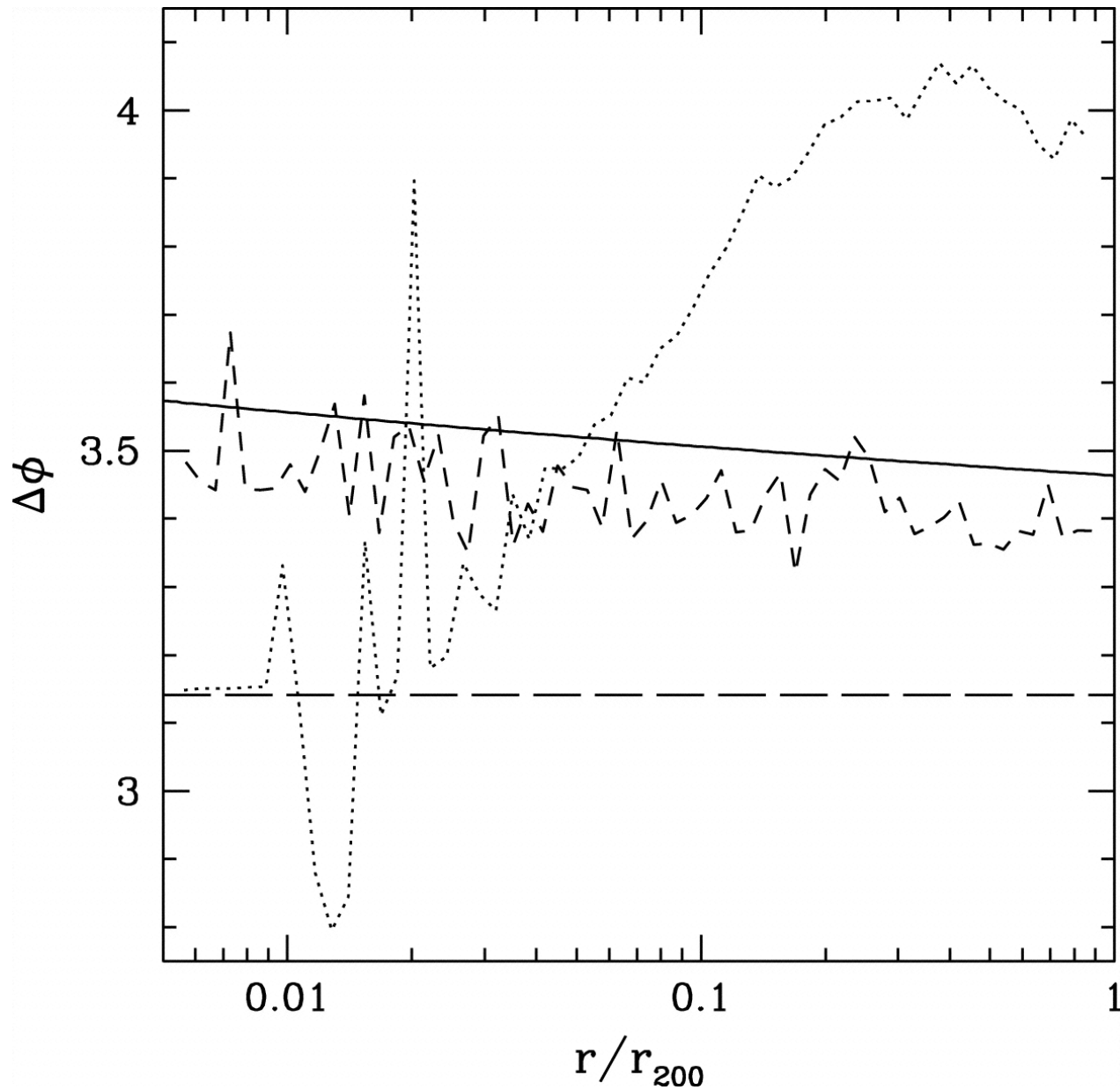
Fig. 11. from On Universal Halos and the Radial Orbit Instability MacMillan, Widrow, & Henriksen 2006 ApJ 653 43 doi:10.1086/508602 https://dx.doi.org/10.1086/508602
