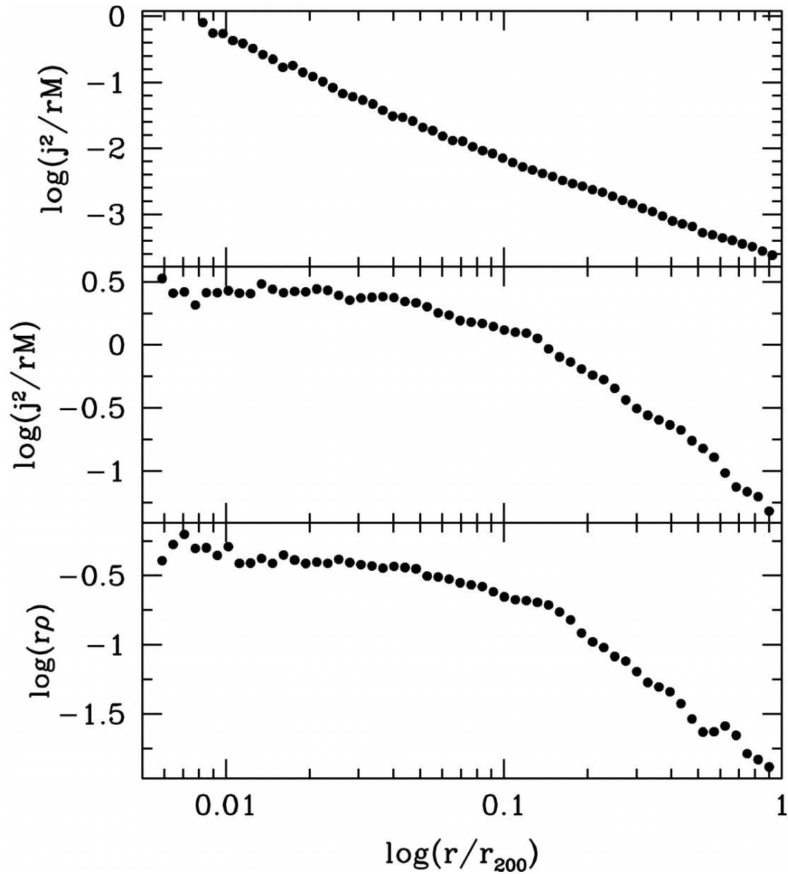
Fig. 10. from On Universal Halos and the Radial Orbit Instability MacMillan, Widrow, & Henriksen 2006 ApJ 653 43 doi:10.1086/508602 https://dx.doi.org/10.1086/508602 © 2006. The American Astronomical Society. All rights reserved. Printed in U.S.A.
