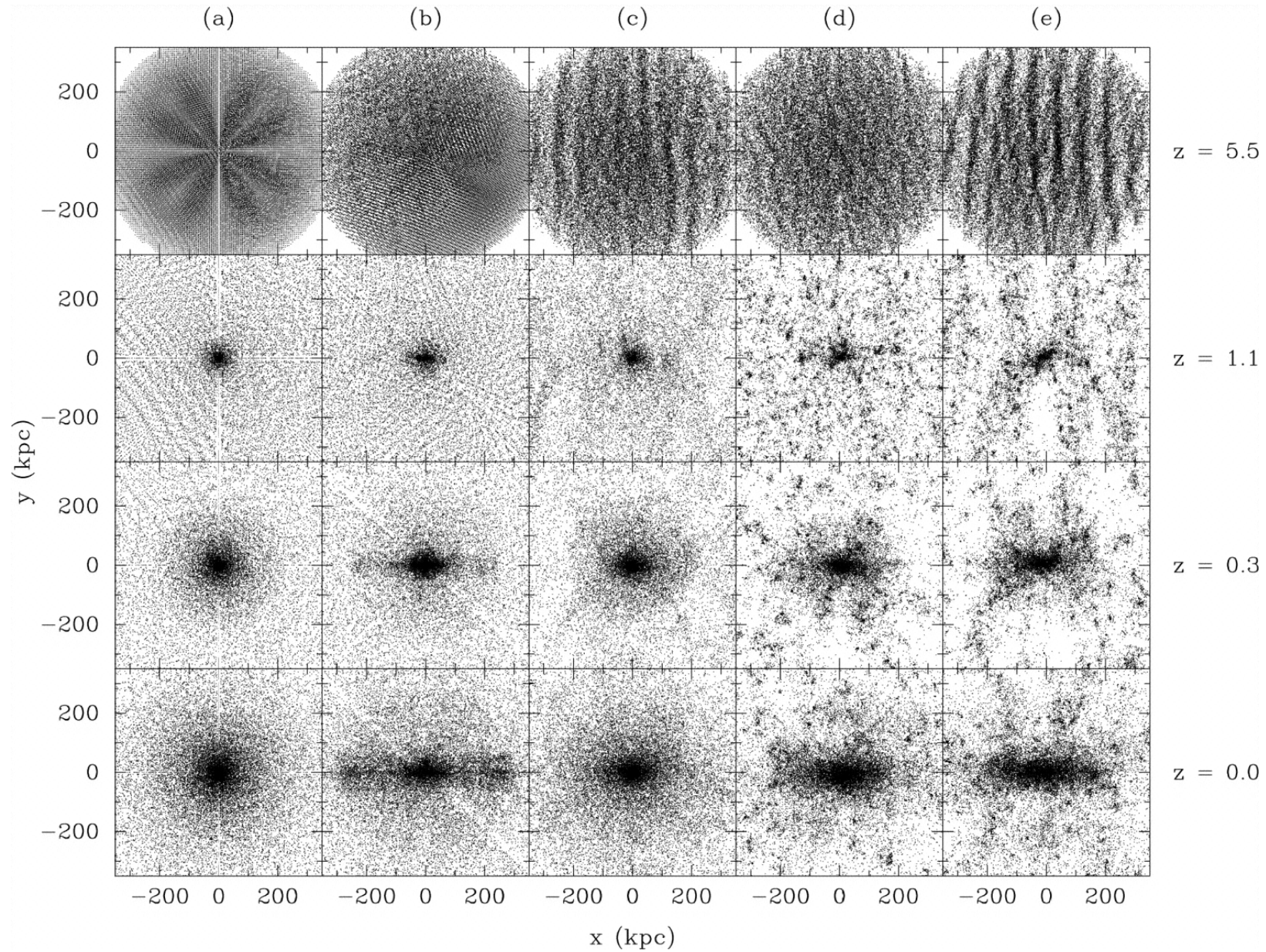
Fig. 1. from On Universal Halos and the Radial Orbit Instability MacMillan, Widrow, & Henriksen 2006 ApJ 653 43 doi:10.1086/508602 https://dx.doi.org/10.1086/508602
