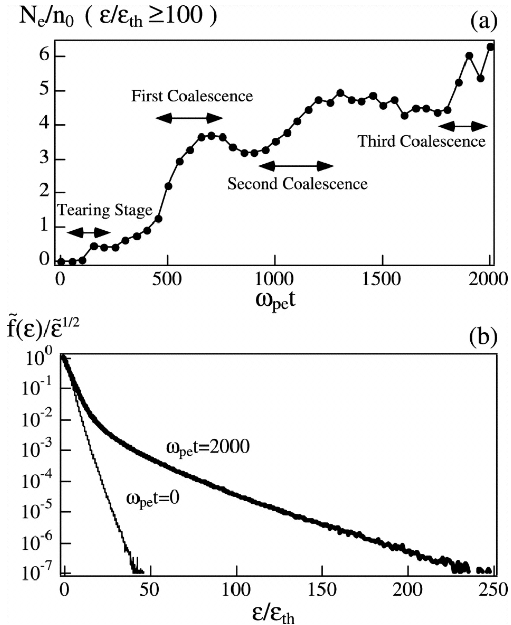
Fig. 8. from A Trigger Mechanism of Magnetic Reconnection and Particle Acceleration during Thinning of the Current Sheet Saito & Sakai 2006 ApJ 652 793 doi:10.1086/508333 https://dx.doi.org/10.1086/508333
