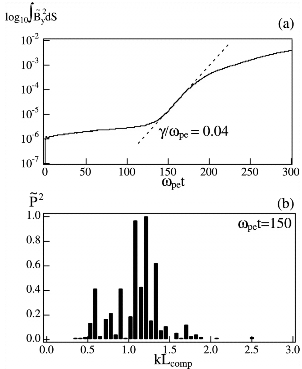
Fig. 6. from A Trigger Mechanism of Magnetic Reconnection and Particle Acceleration during Thinning of the Current Sheet Saito & Sakai 2006 ApJ 652 793 doi:10.1086/508333 https://dx.doi.org/10.1086/508333 © 2006. The American Astronomical Society. All rights reserved. Printed in U.S.A.
